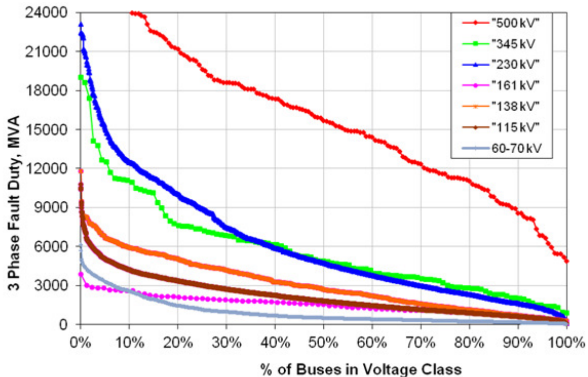
Figure 1: WECC Bus Three Phase Short Circuit MVA 2009HS3 Base Case
