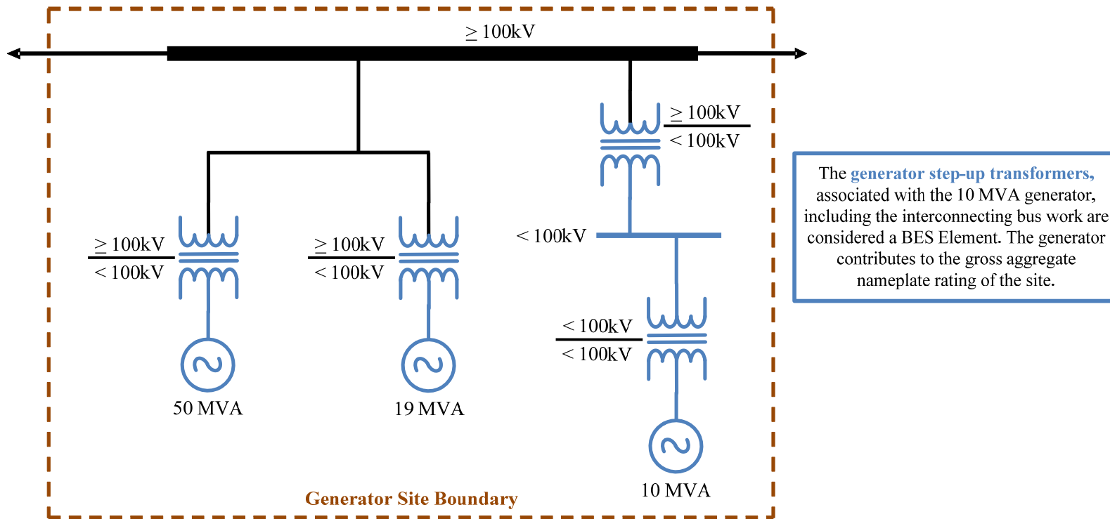
Figure I2-5: Multiple Generators at a Single Site (BES)
