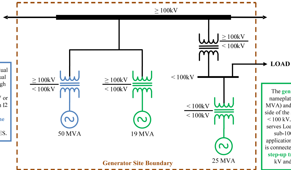
Figure I2-6: Multiple Generators at a Single Site (BES & non-BES)
