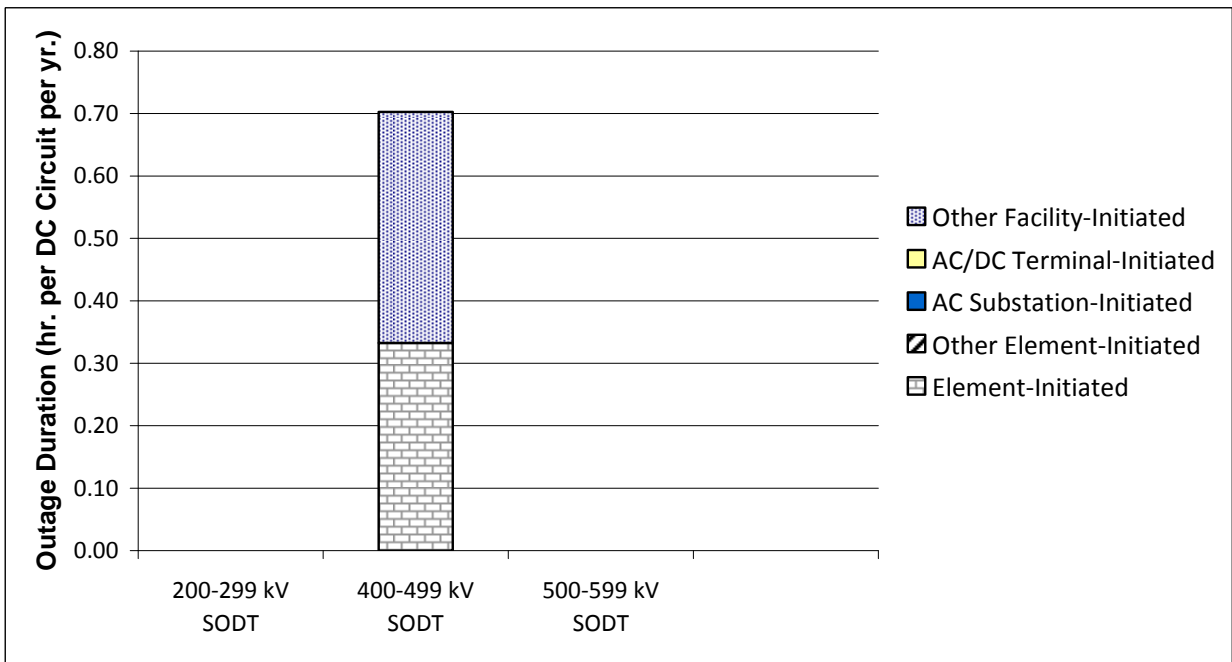
Figure MRO 2-4 DC Circuit Outage Duration by Outage Initiation Code
