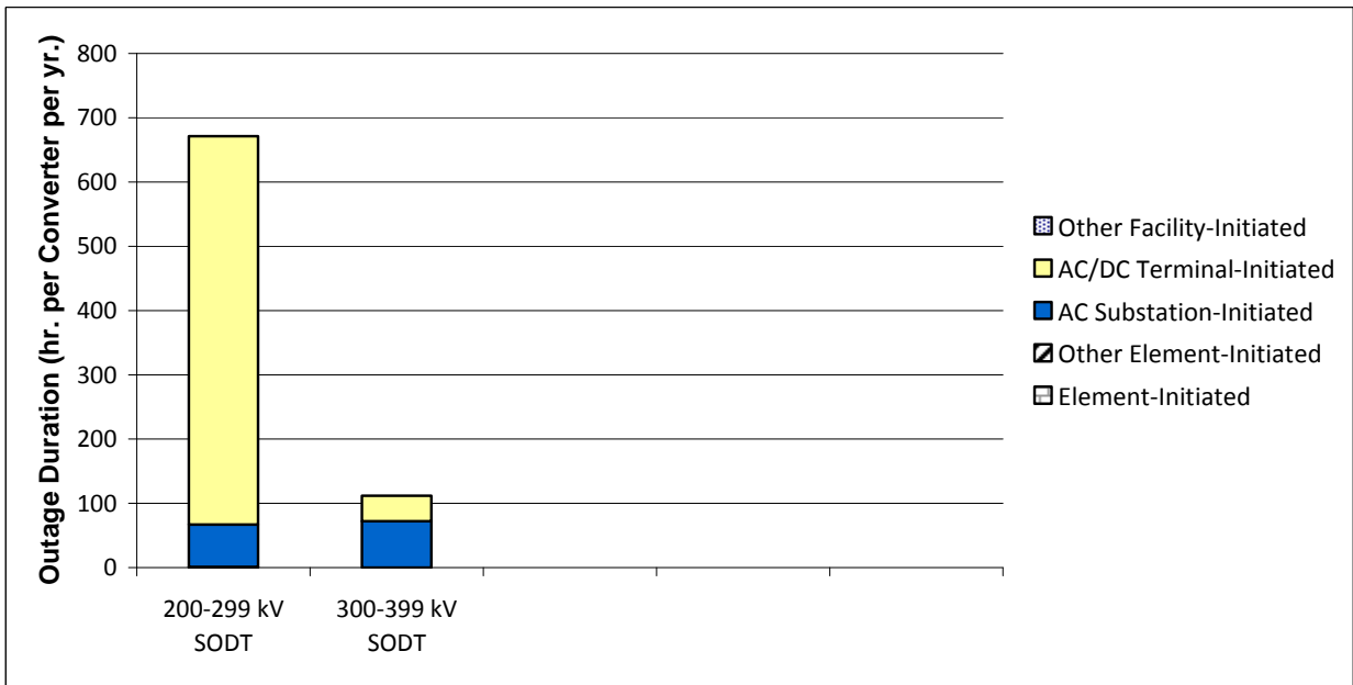
Figure WECC 2-8 AC/DC BTB Converter Outage Duration by Outage Initiation Code
