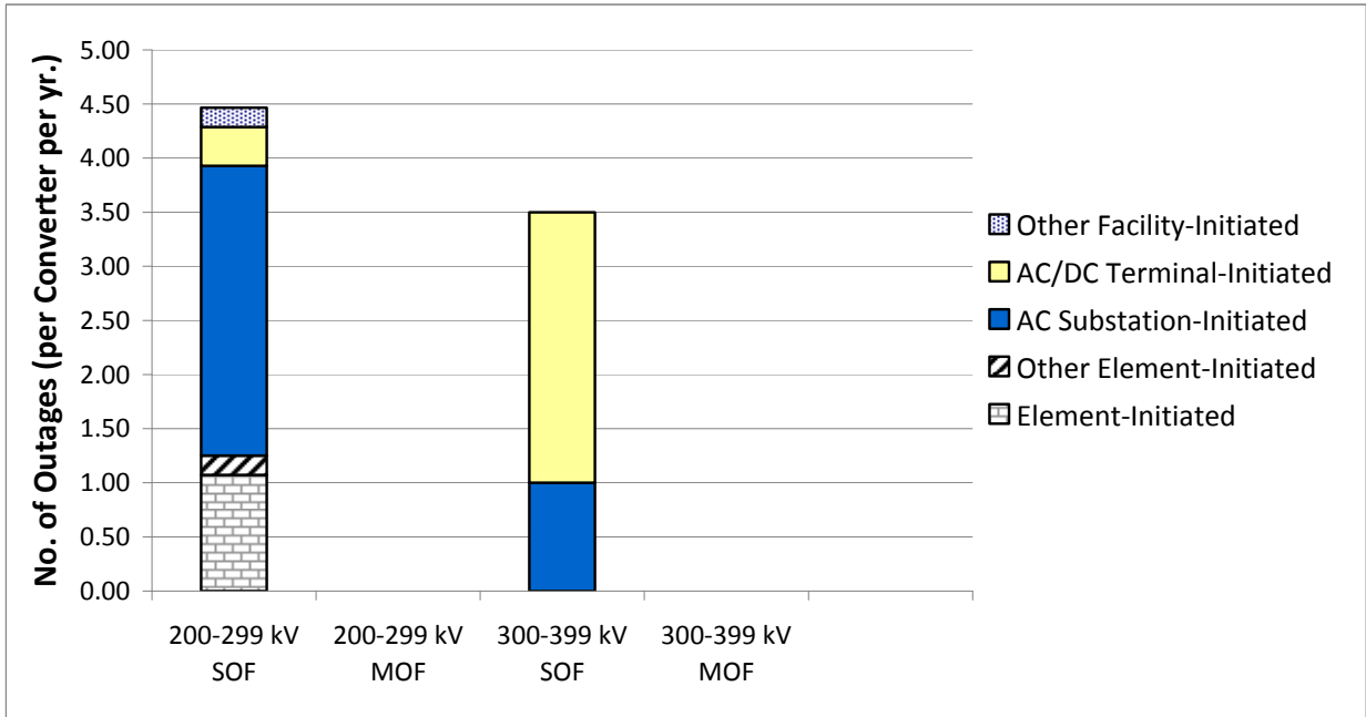
Figure WECC 2-7 AC/DC BTB Converter Outage Frequency by Outage Initiation Code
