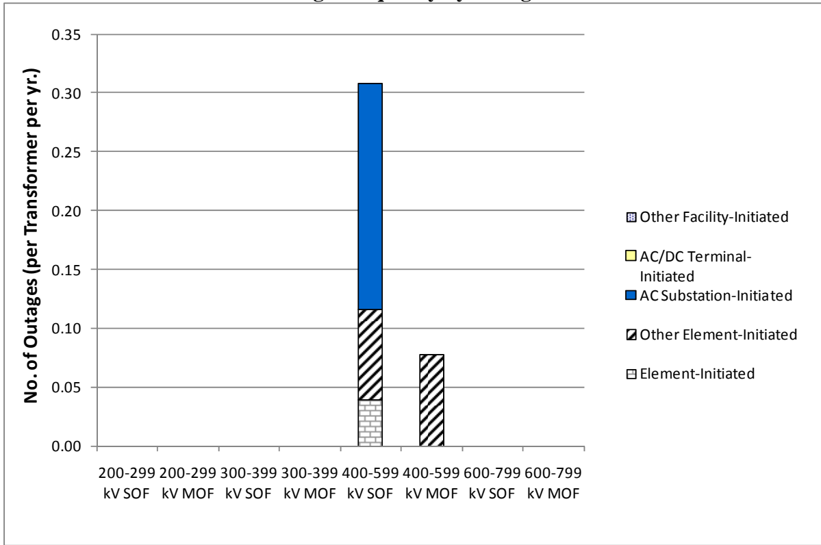
Figure FRCC 2-5 Transformer Outage Frequency by Outage Initiation Code
