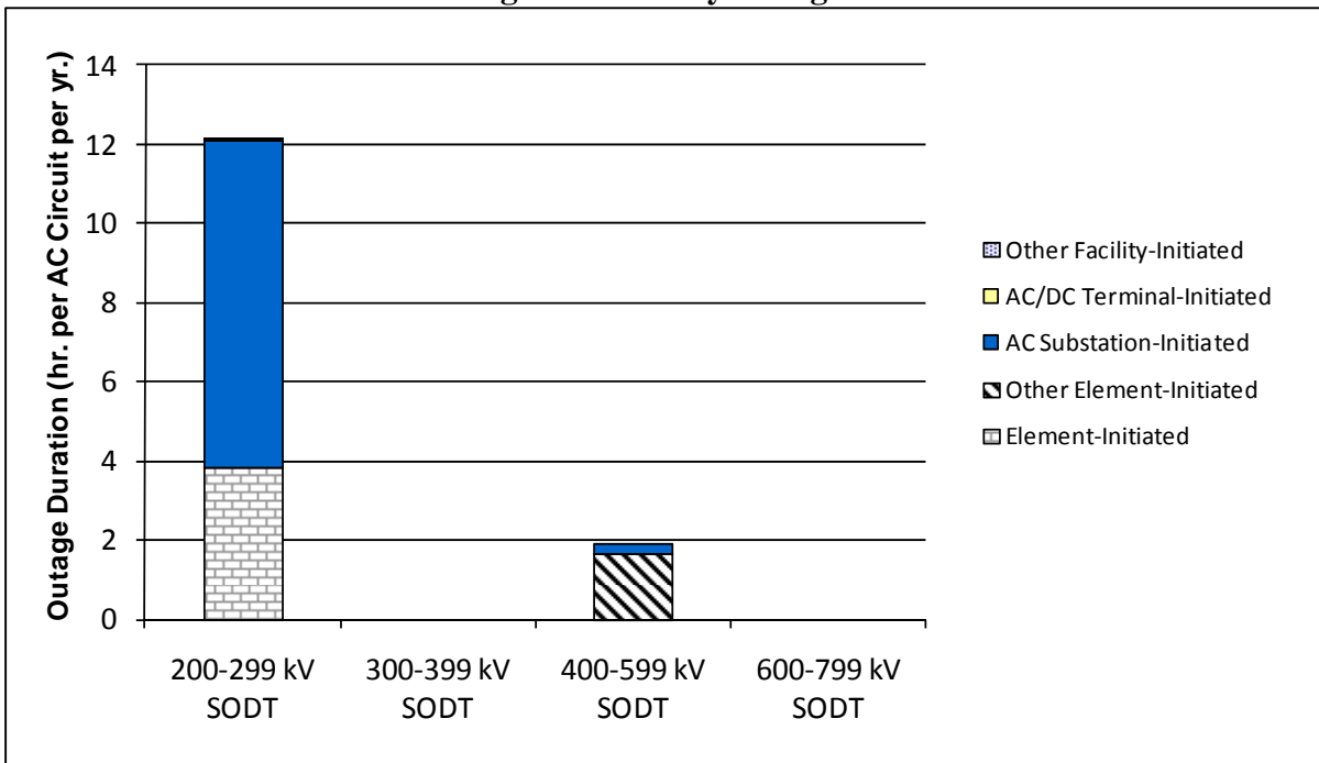
Figure FRCC 2-2 AC Circuit Outage Duration by Outage Initiation Code
