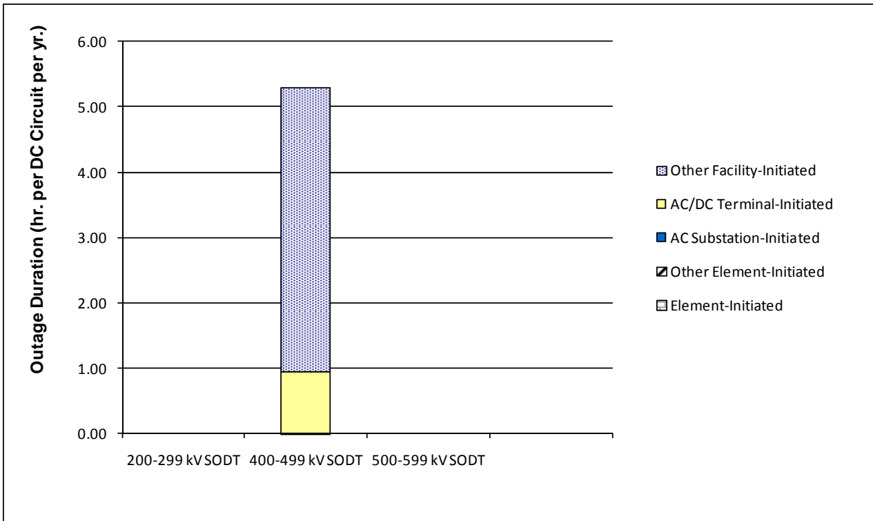
Figure MRO 2-4 DC Circuit Outage Duration by Outage Initiation Code
