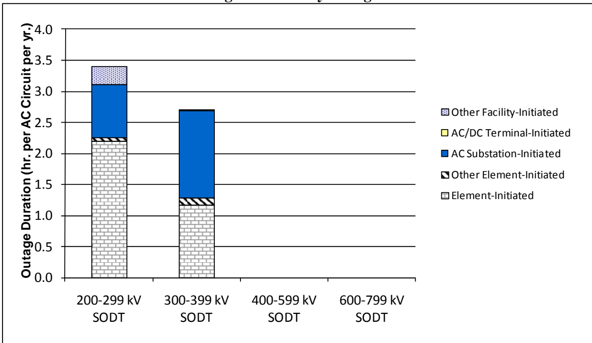
Figure MRO 2-2 AC Circuit Outage Duration by Outage Initiation Code
