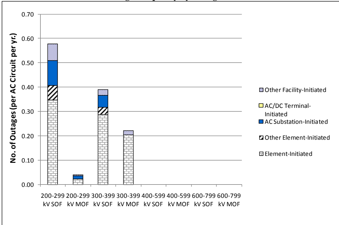
Figure MRO 2-1 AC Circuit Outage Frequency by Outage Initiation Code
