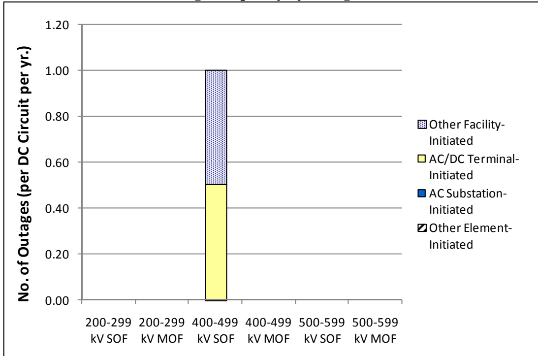
Figure MRO 2-3 DC Circuit Outage Frequency by Outage Initiation Code
