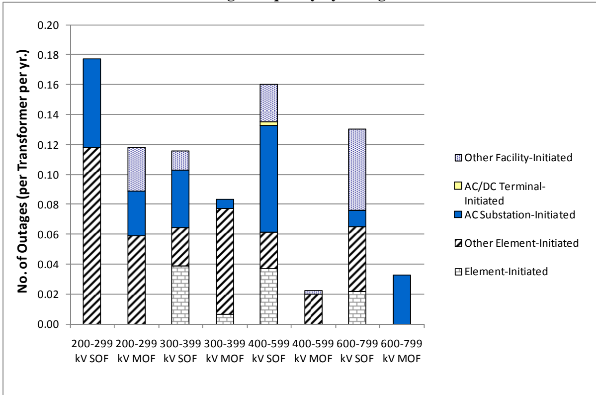
Figure NERC 2-5 Transformer Outage Frequency by Outage Initiation Code
