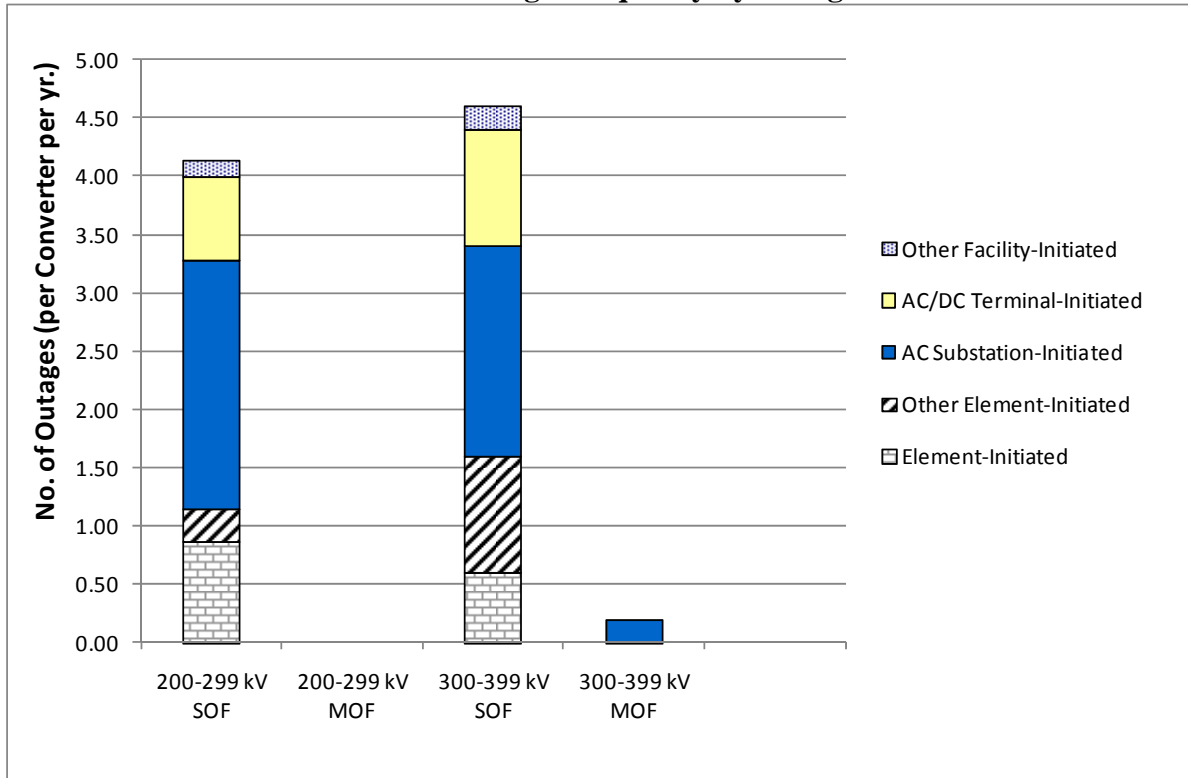
Figure NERC 2-7 AC/DC BTB Converter Outage Frequency by Outage Initiation Code
