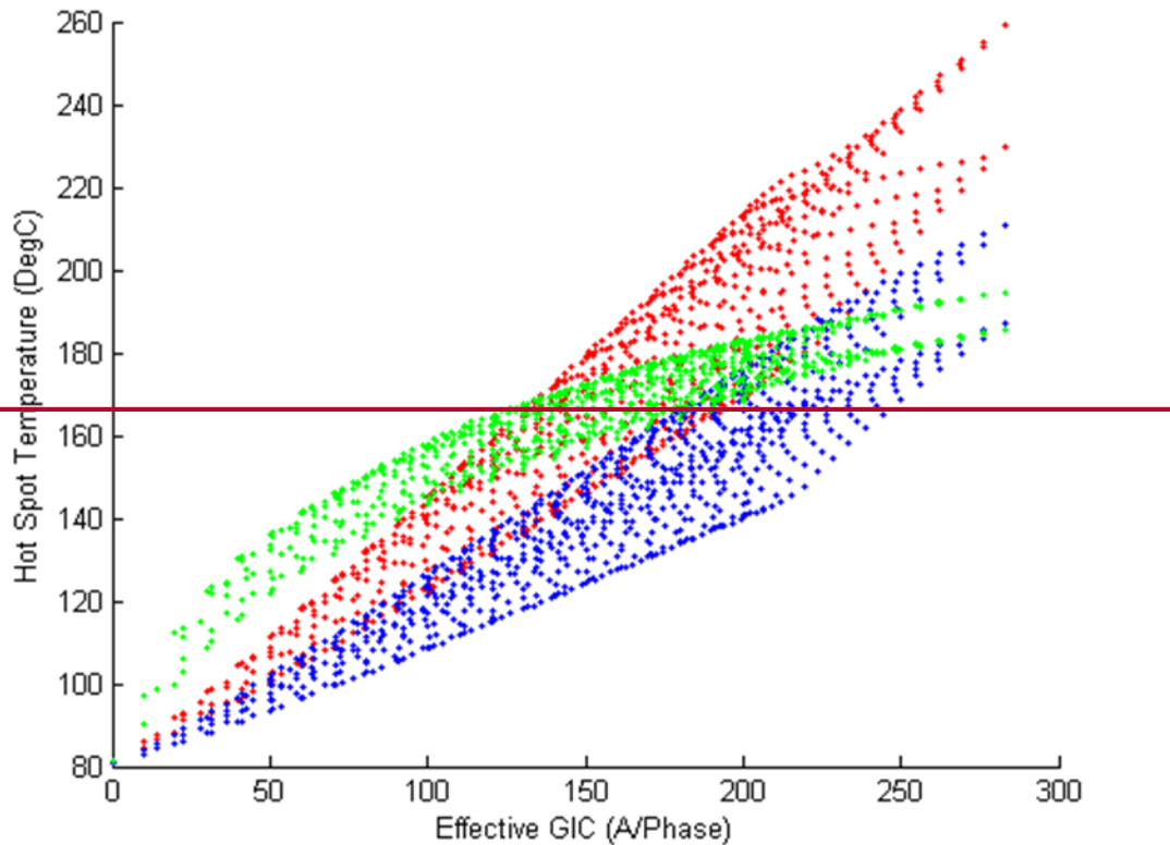
Figure 1: Metallic hot spot temperatures calculated using the benchmark GMD event. Red: Screening model [2]. Blue: Fingrid model [3]. Green: SoCo model [4]. [A1]
