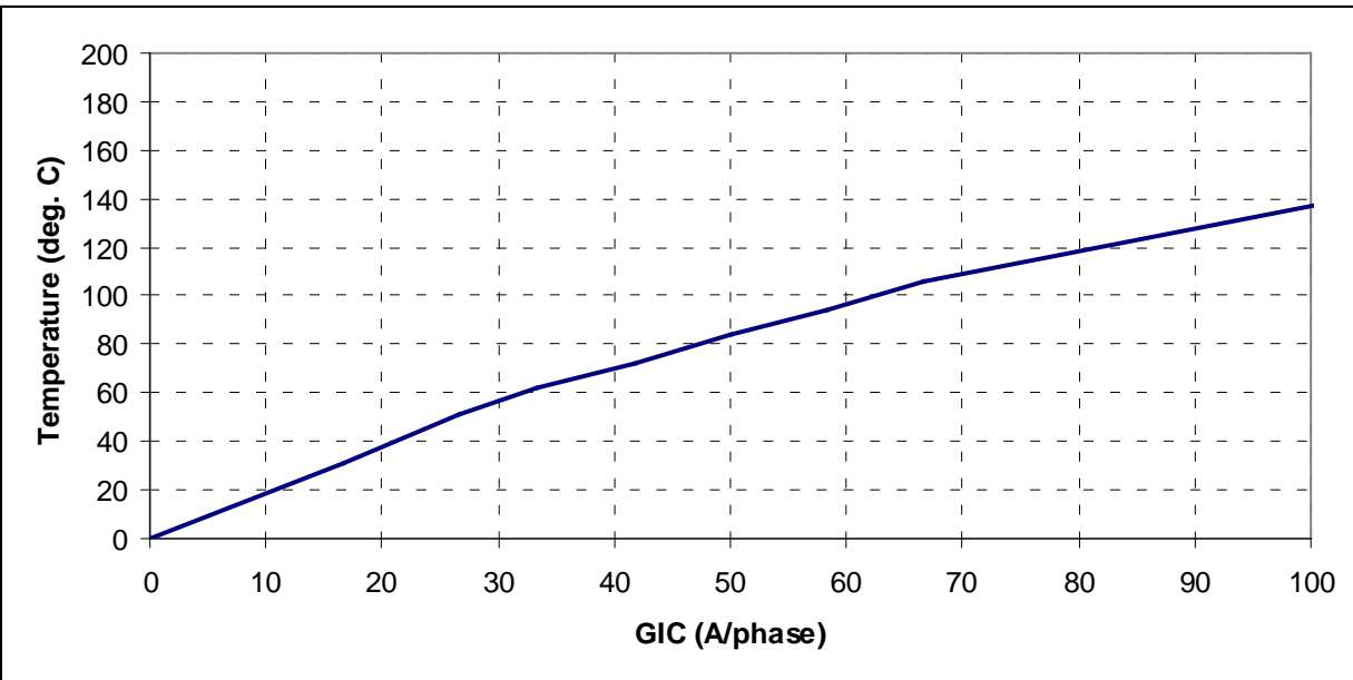
Figure 45: Asymptotic thermal response of the inside of top yoke clamp Fitch plate of a 400 kV 400 MVA five-leg core-type fully-wound transformer.
