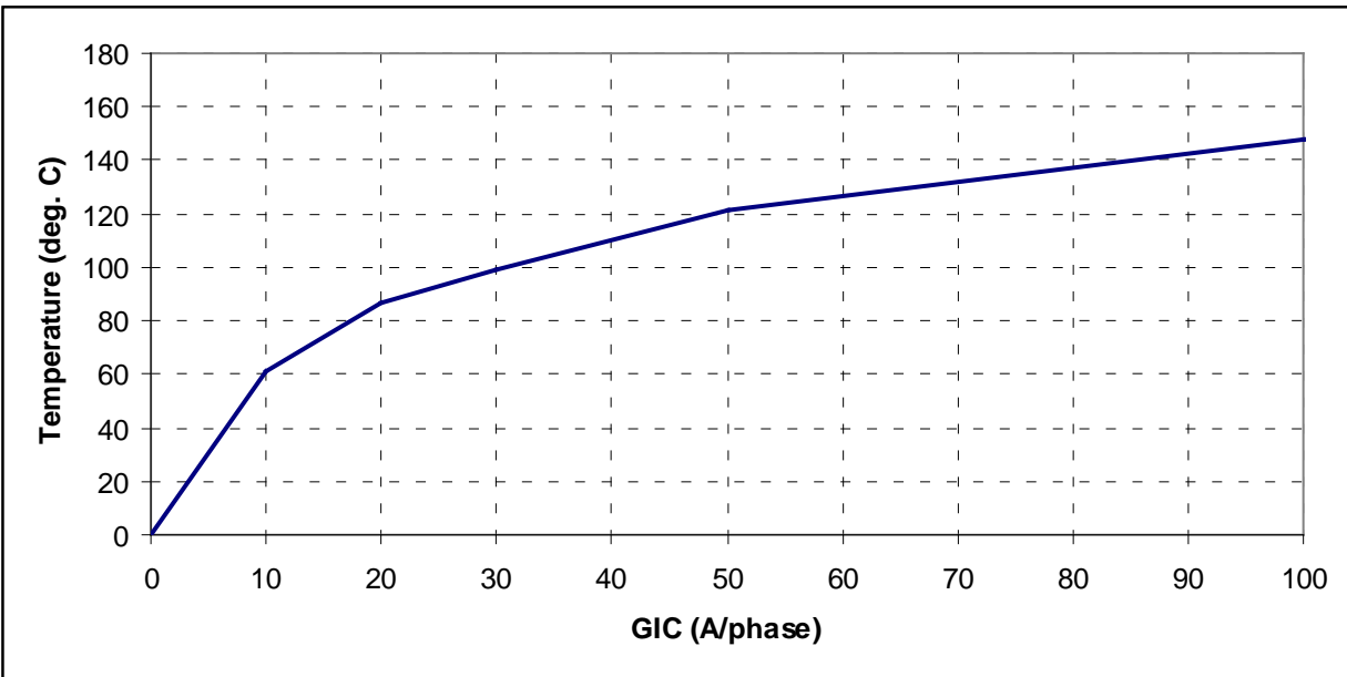
Figure 67: Asymptotic thermal response of the Flitch plate of a 400 kV 400 MVA single-phase core-type autotransformer.
