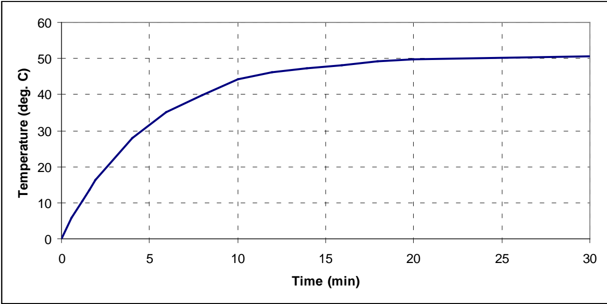
Figure 56: Step thermal response of tie plate of a 400 kV 400 MVA single-phase core-type autotransformer to a 10 A per phase dc step.
