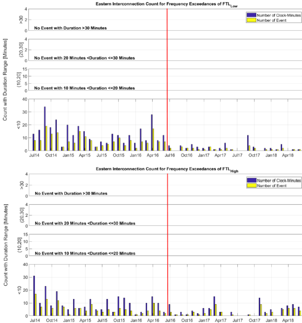
Figure 2.2: Eastern Interconnection FTL Exceedances
