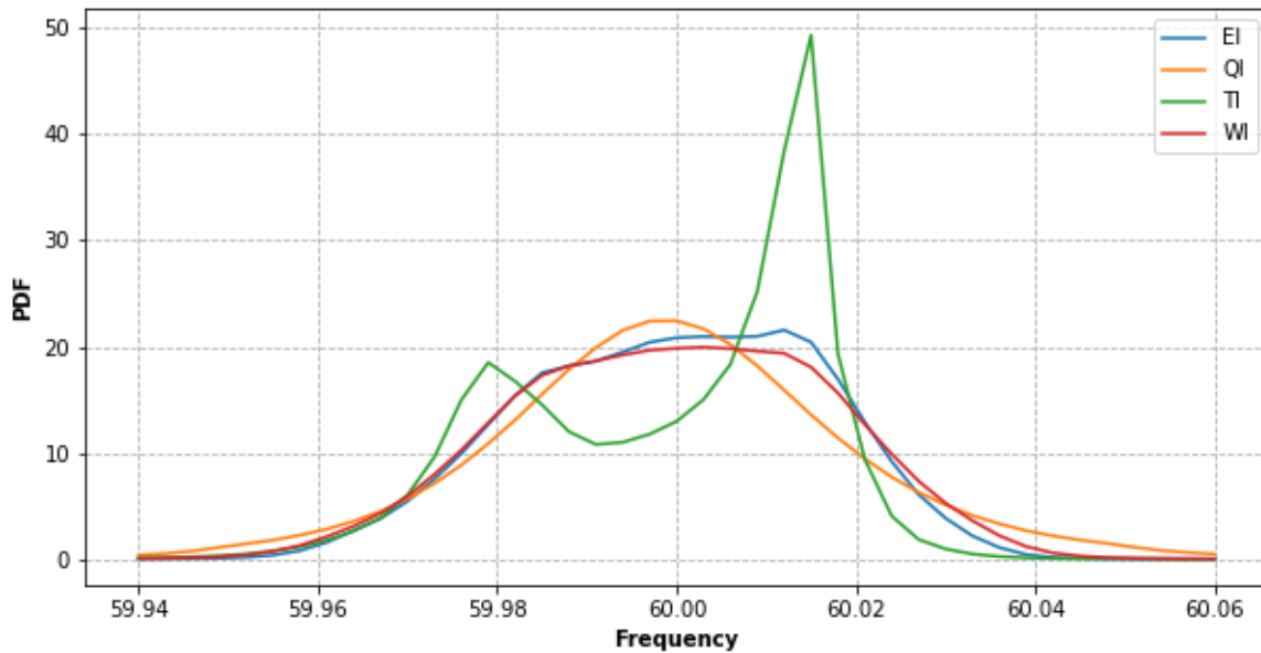
Figure 1.5: Comparison of 2018–2022 Interconnection Frequency PDFs
