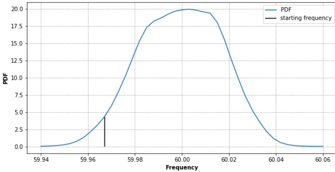
Figure 1.2: Western Interconnection 2018–2022 Probability Density Function of Frequency
