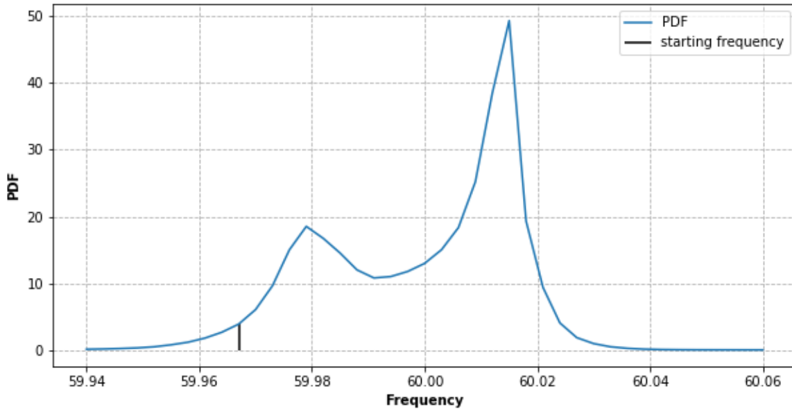
Figure 1.3: Texas Interconnection 2018–2022 Probability Density Function of Frequency
