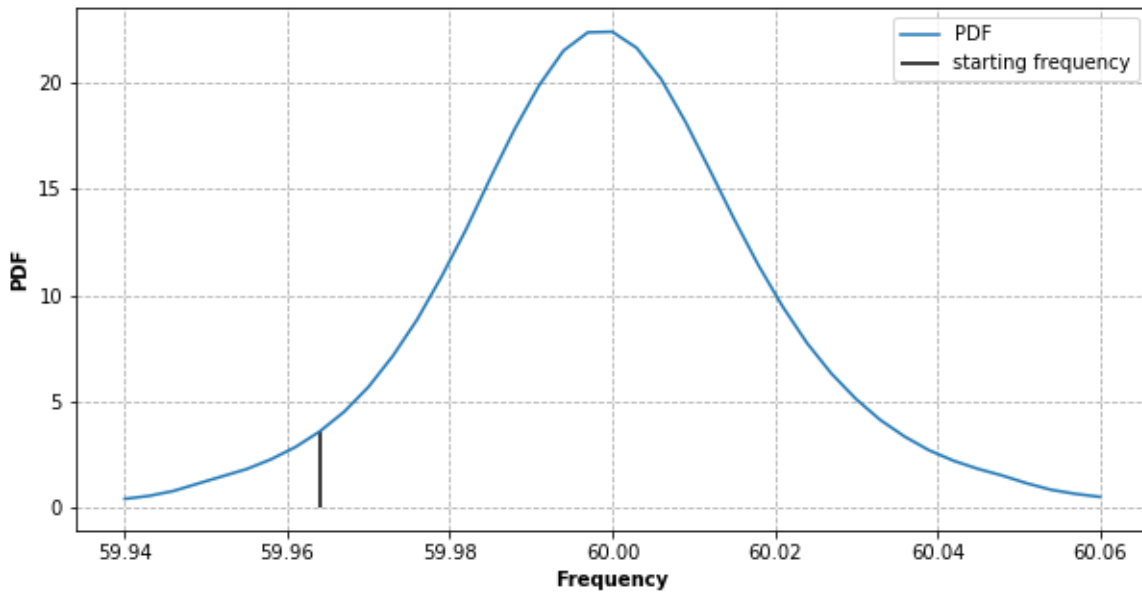
Figure 1.4: Québec Interconnection 2018–2022 Probability Density Function of Frequency
