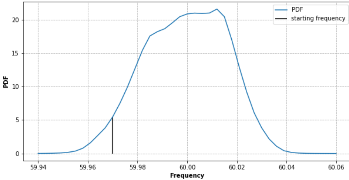
Figure 1.1: Eastern Interconnection 2018–2022 Probability Density Function of Frequency
