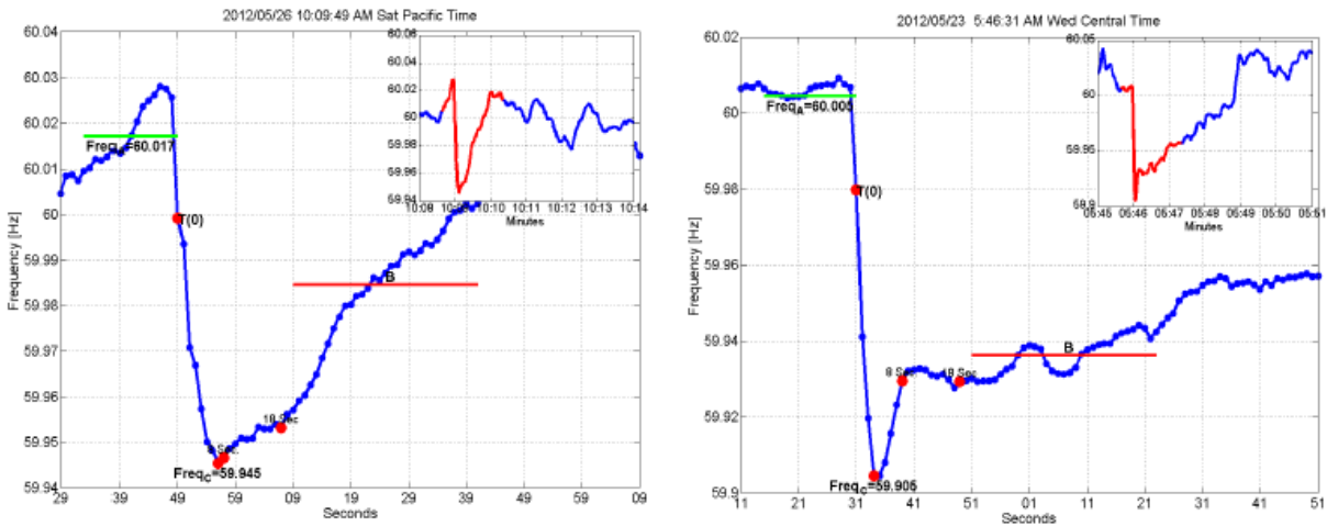
Figure 1.1: Pre-disturbance Frequency
