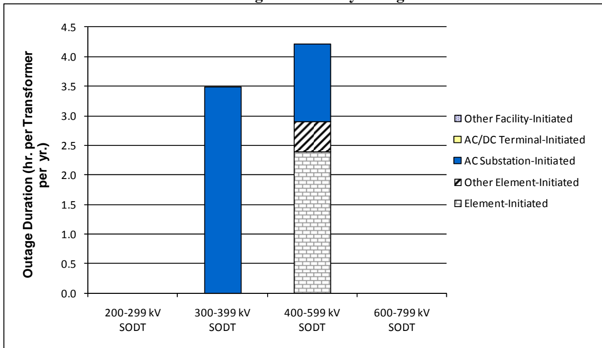
Figure MRO 2-6 Transformer Outage Duration by Outage Initiation
