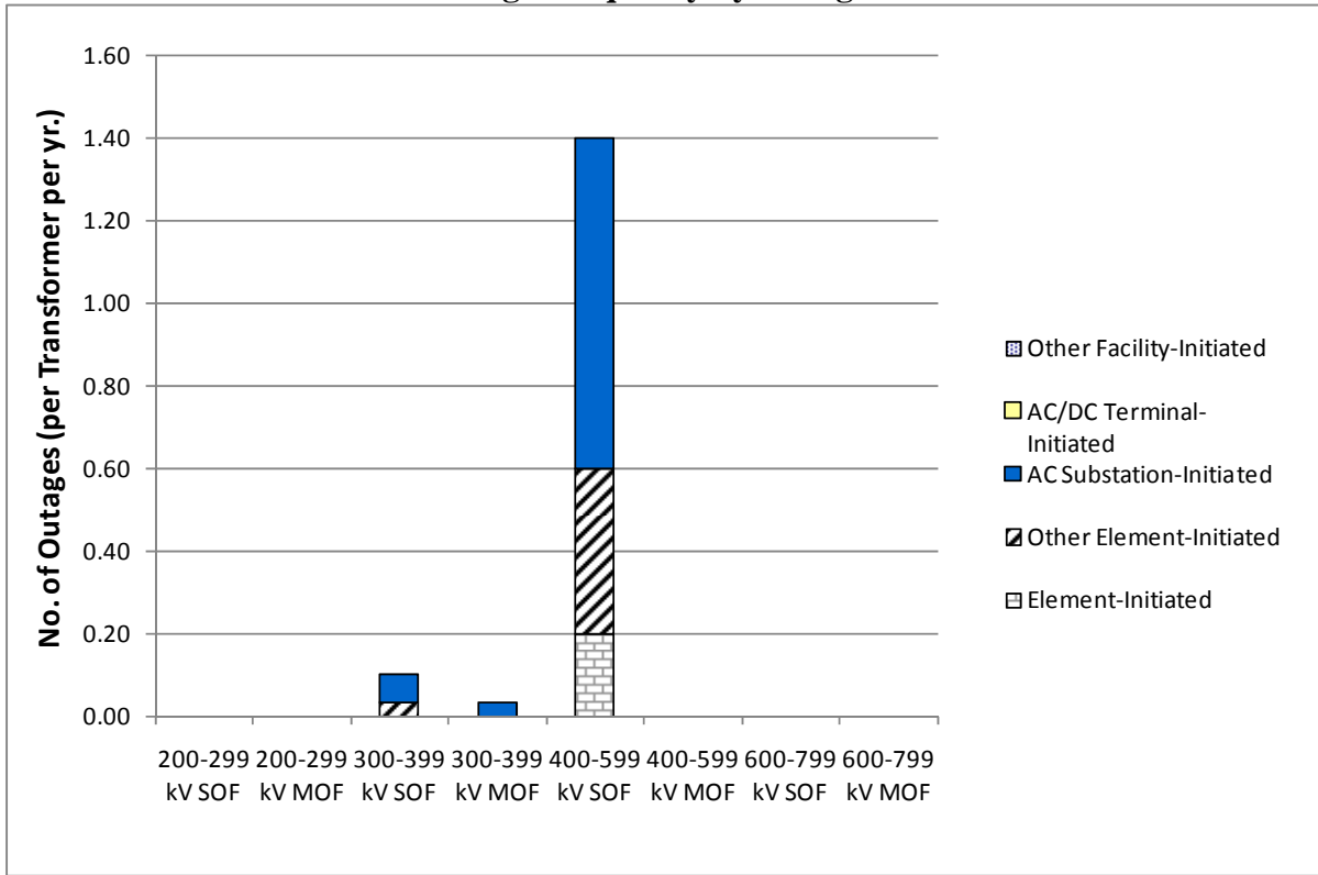
Figure MRO 2-5 Transformer Outage Frequency by Outage Initiation Code
