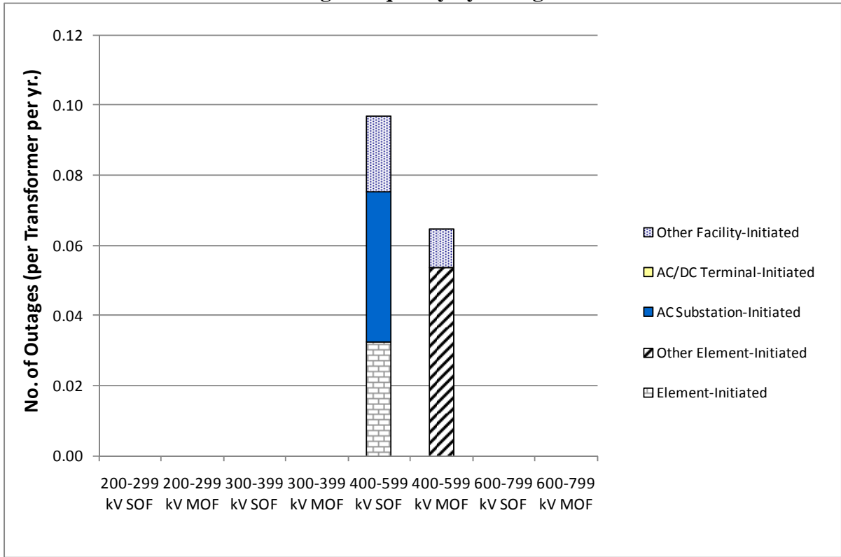
Figure SERC 2-5 Transformer Outage Frequency by Outage Initiation Code
