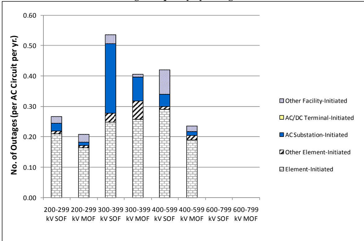
Figure SERC 2-1 AC Circuit Outage Frequency by Outage Initiation Code
