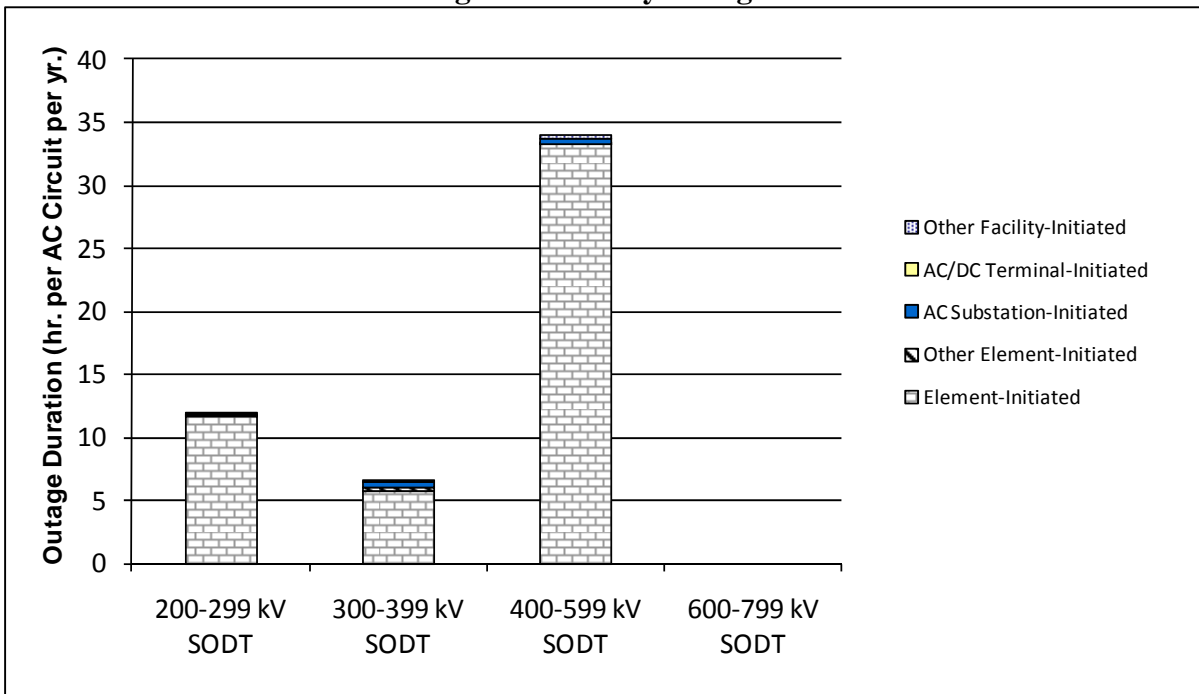
Figure SERC 2-2 AC Circuit Outage Duration by Outage Initiation Code
