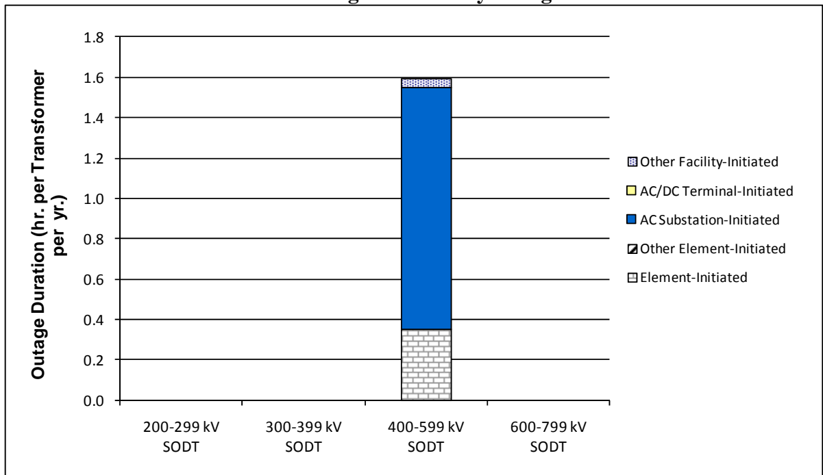
Figure SERC 2-6 Transformer Outage Duration by Outage Initiation
