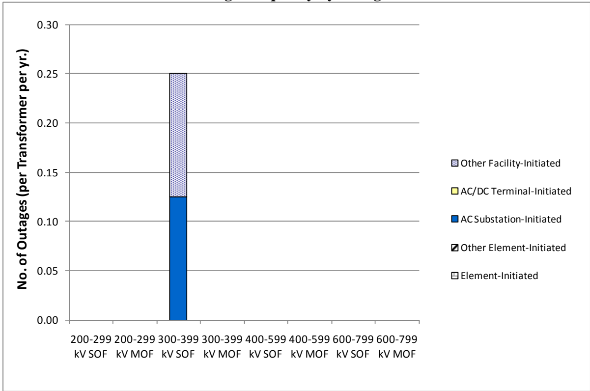
Figure SPP 2-5 Transformer Outage Frequency by Outage Initiation Code
