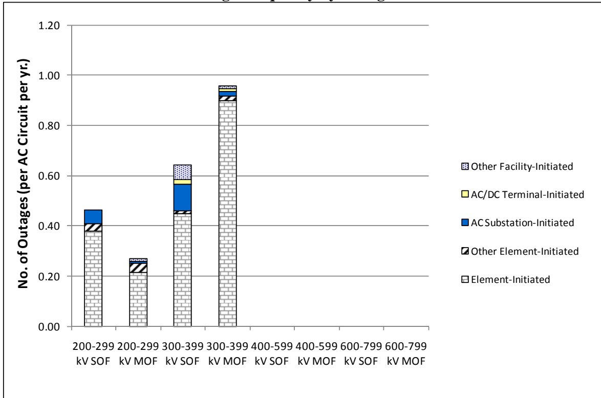
Figure SPP 2-1 AC Circuit Outage Frequency by Outage Initiation Code
