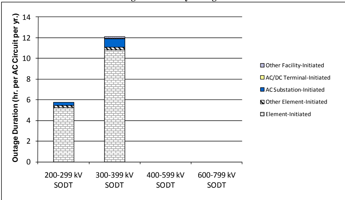
Figure SPP 2-2 AC Circuit Outage Duration by Outage Initiation Code
