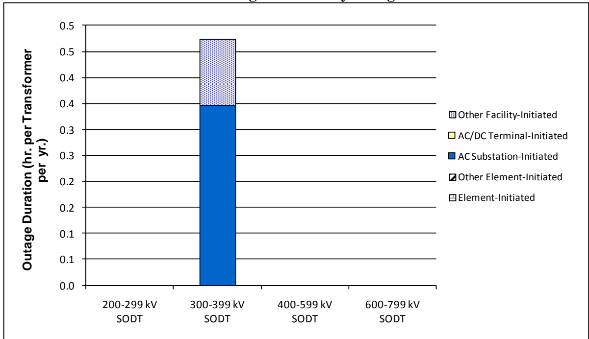
Figure SPP 2-6 Transformer Outage Duration by Outage Initiation
