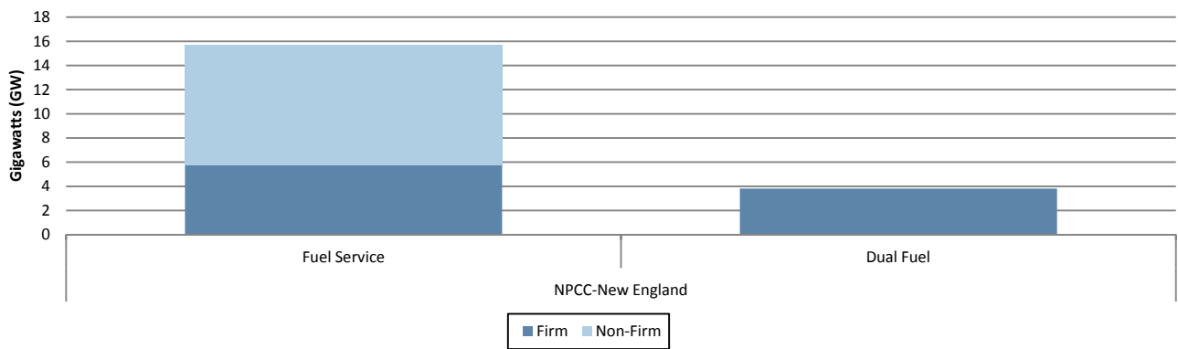
Figure 6: Natural Gas Fuel Service for NPCC-New England
