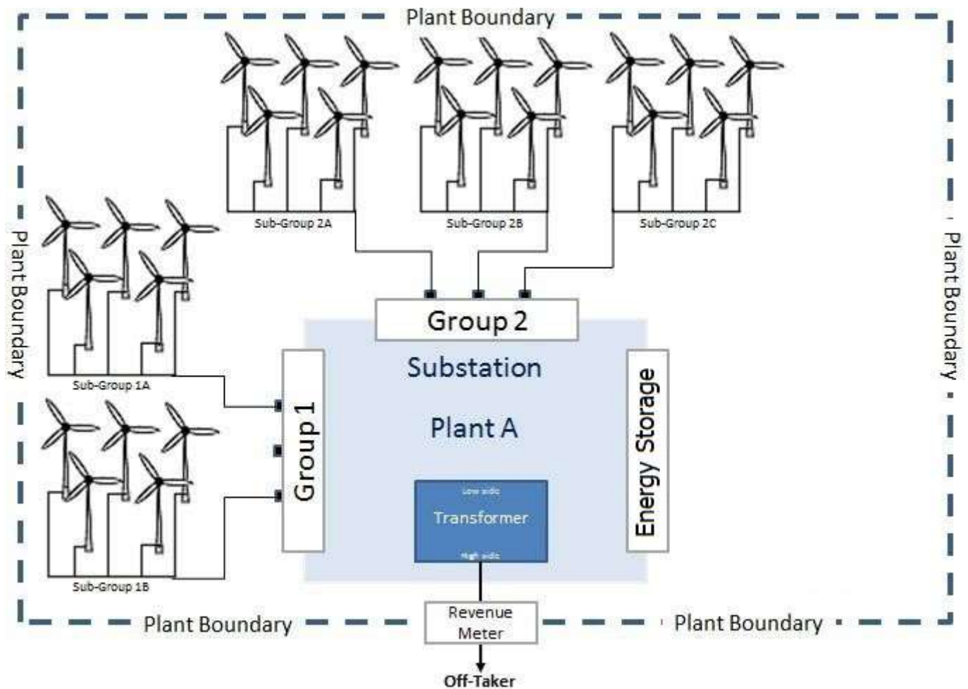
Figure 2.1: Typical Wind Plant Layout
