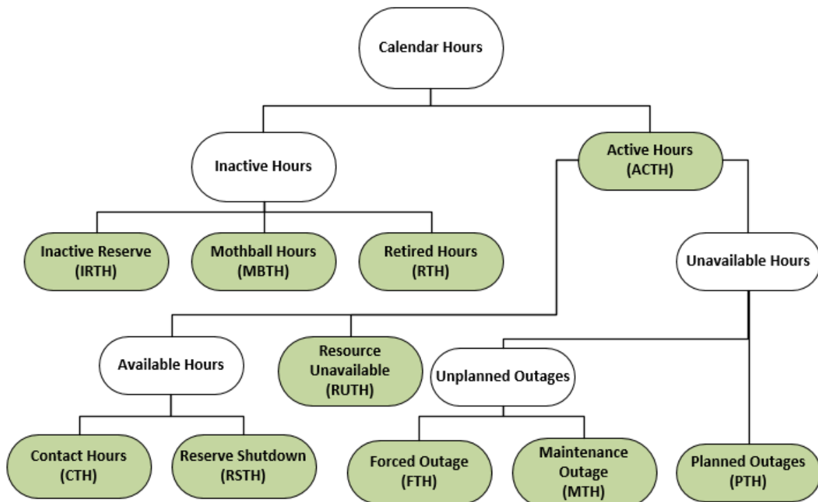
Figure G.1: Time Spent in Various Turbine Unit States
