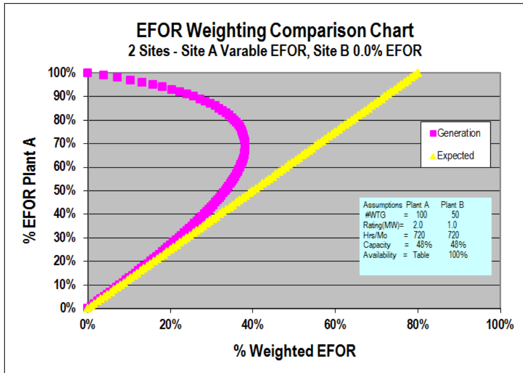
Figure L.3: Percent of Weighted EFOR
