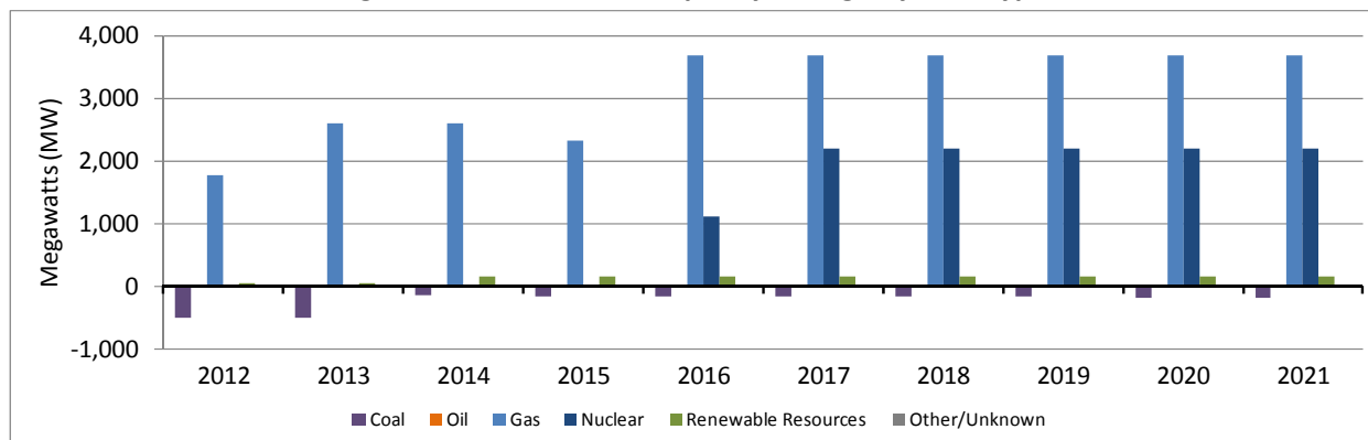
Figure 117: Annual Net Capacity Change by Fuel Type
