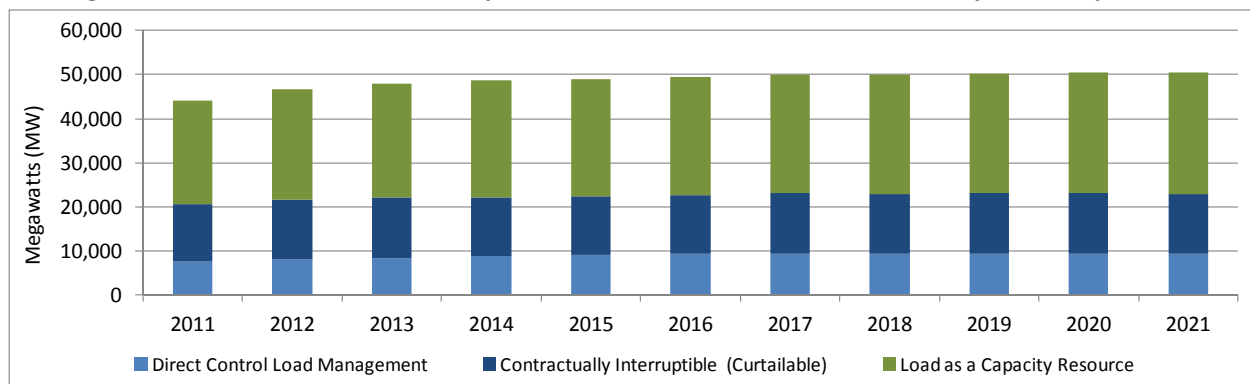
Figure 15: NERC-Wide On-Peak Dispatchable and Controllable Demand Response Projections
