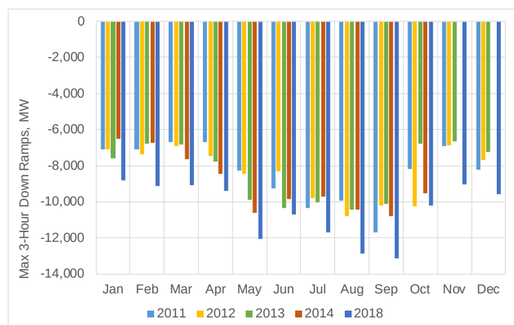
Figure B.3b: Max. monthly three-hour down ramps
