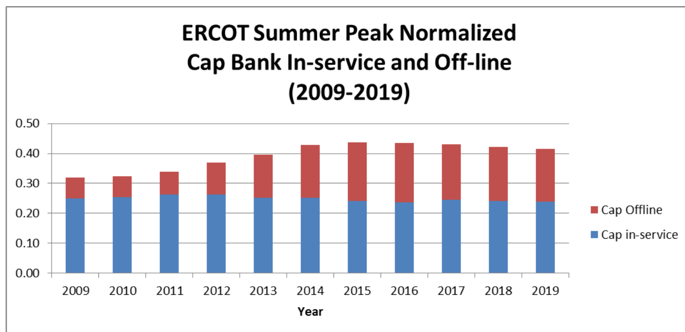
Figure D.53: ERCOT – Planning – Static System (p.u.) (Summer Peak)
