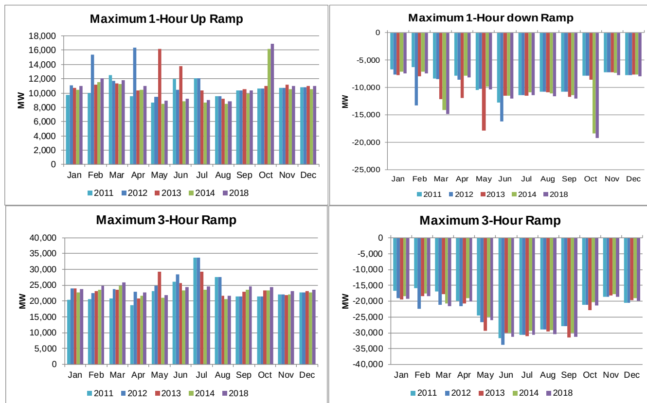
Figure B.20: PJM Maximum 1- and 3-hour net load up and down ramps
