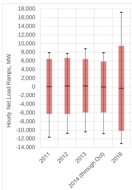
Figure B.3c: Yearly three-hour ramp distribution
