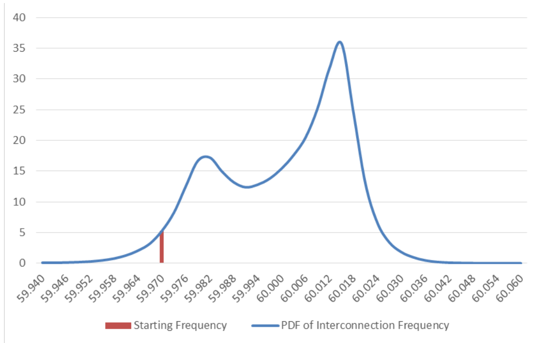
Figure 1.3: Texas Interconnection 2015–2018 Probability Density Function of Frequency
