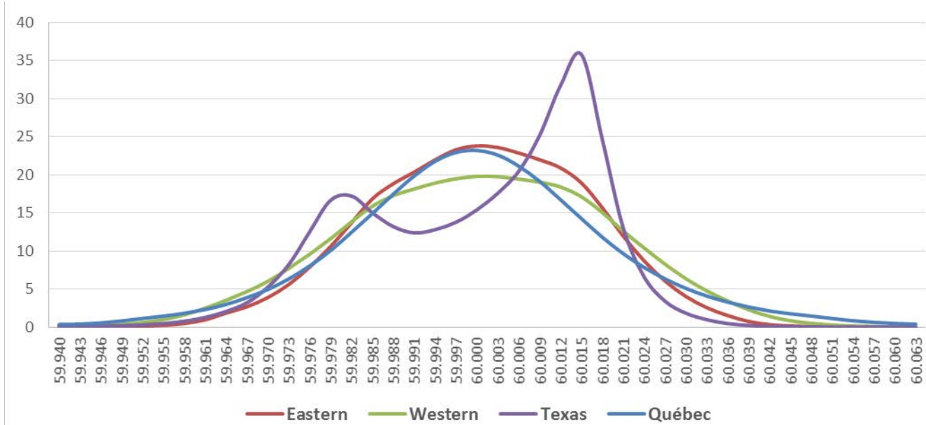
Figure 1.5: Comparison of 2015–2018 Interconnection Frequency PDFs
