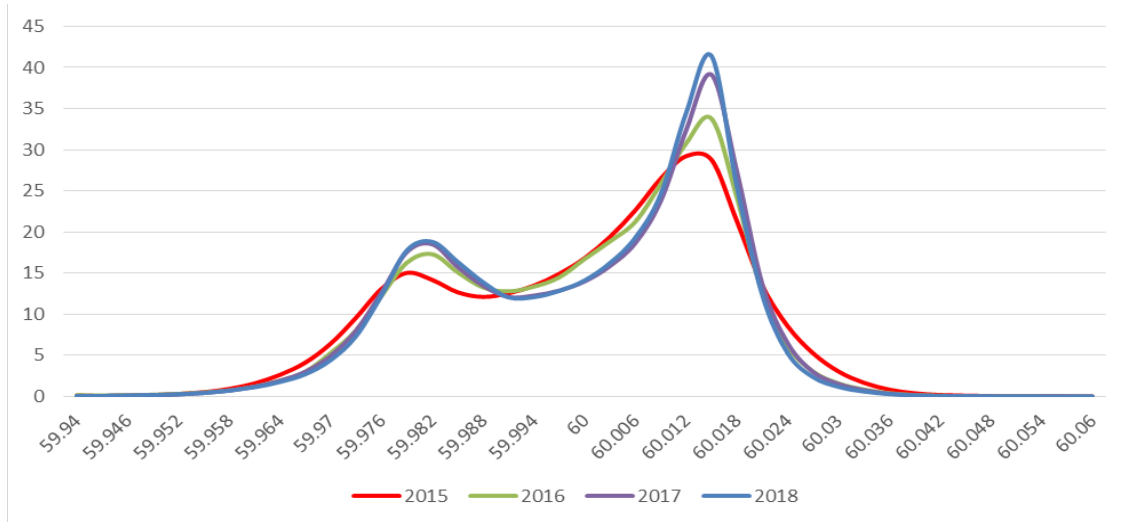
Figure 1.8: Texas Interconnection Frequency Probability Density Function by Year
