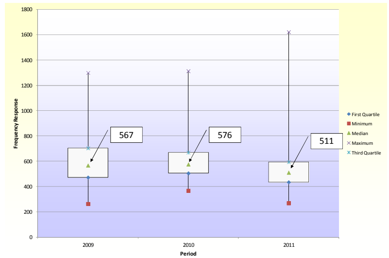
Figure H5 – ERCOT Interconnection Frequency Response Analysis for 2009 to 2011
