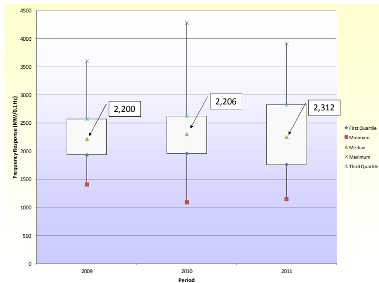
Figure H3 – Eastern Interconnection Frequency Response Analysis for 2009 to 2011
