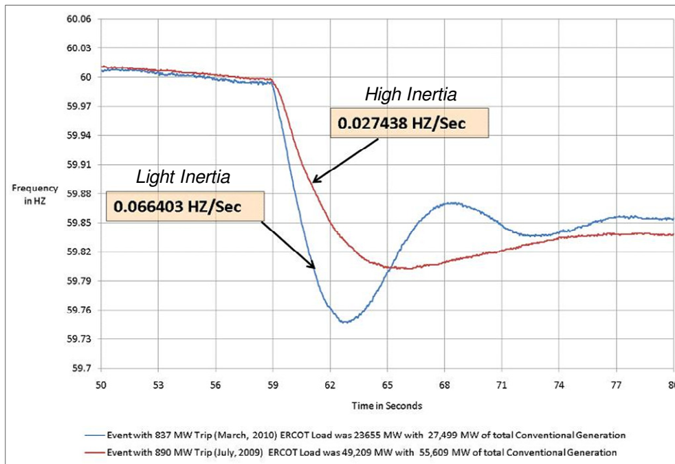
Figure YYY: Inertial Response Sensitivity
