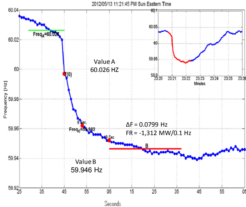
Figure E2 – 11:21 pm Sunday Night 1,049 MW Resource Loss
