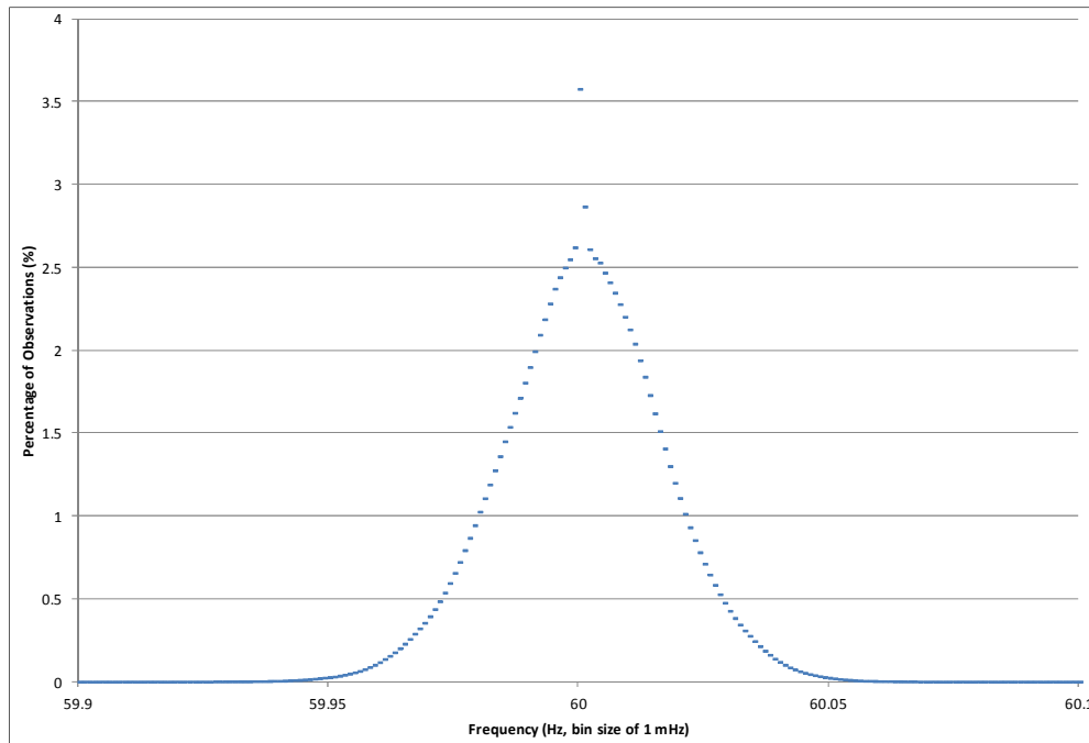
Figure FA1 Eastern Interconnection 2007-2011 Frequency Histogram
