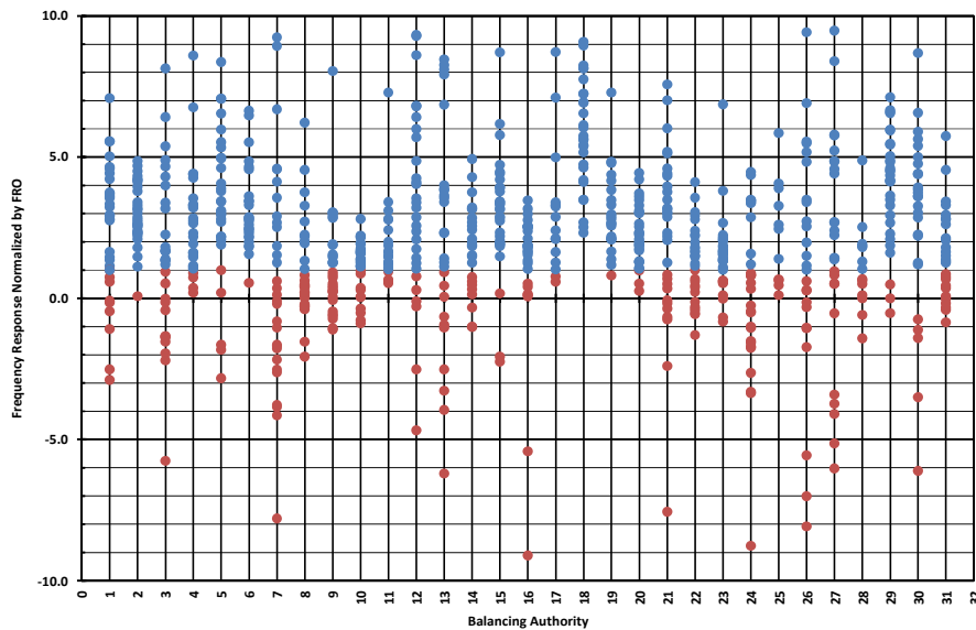
Figure H1 – 2011 Normalized Frequency Response Events by BA Eastern Interconnection
