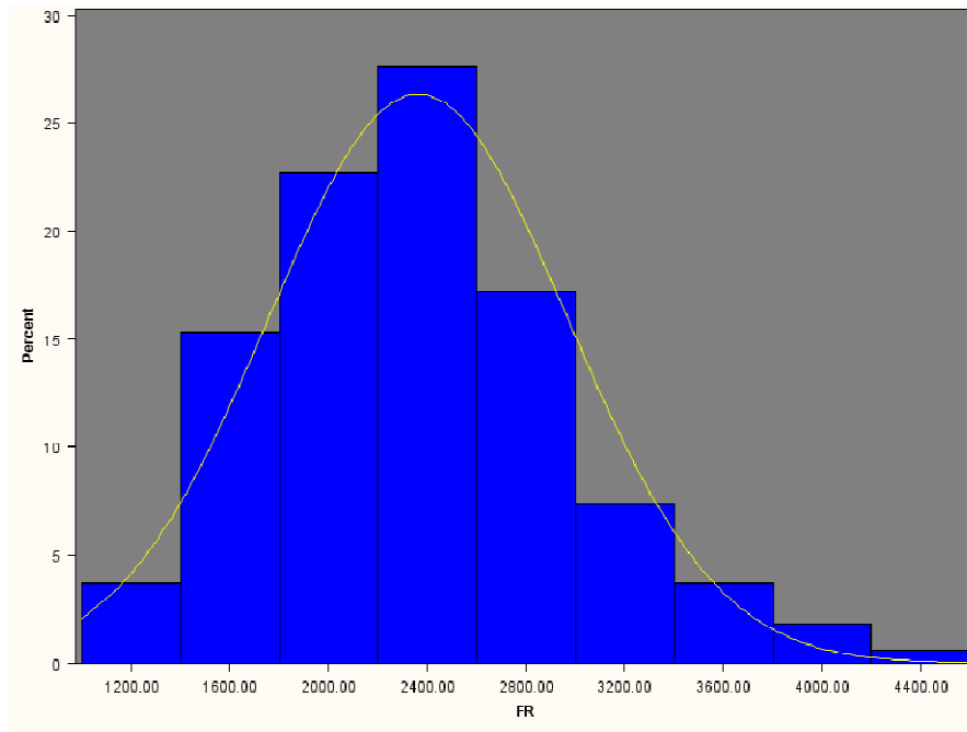
Figure Stat2: Probability Distribution Eastern Interconnection Frequency Response 2009 through April 2012
