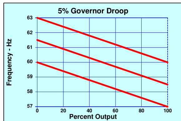
Figure Droop 1 – Sample Droop Characteristic Curve
