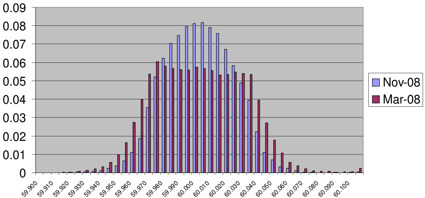
Figure T3 – Comparison of Frequency Profiles for November and March 2008 (in 5 mHz bins)
