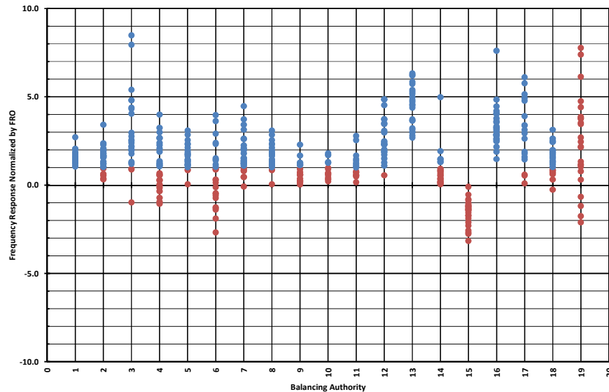
Figure H2 – 2011 Normalized Frequency Response Events by BA Western Interconnection
