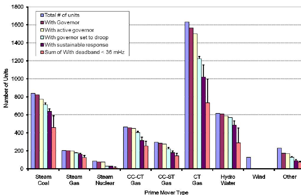
Figure S1 – Eastern Interconnection Generator Responses
