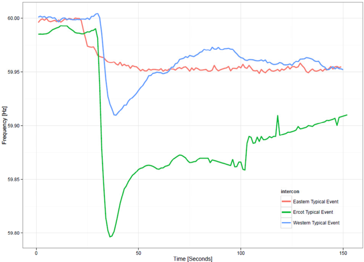
Figure SS -- Typical Interconnection Responses for 2011
