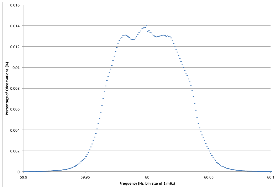
Figure FA3: ERCOT Interconnection 2007-2011 Frequency Histogram
