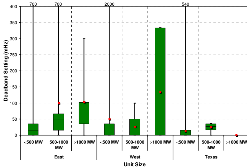
Figure S7 – Reported Governor Deadband Settings
