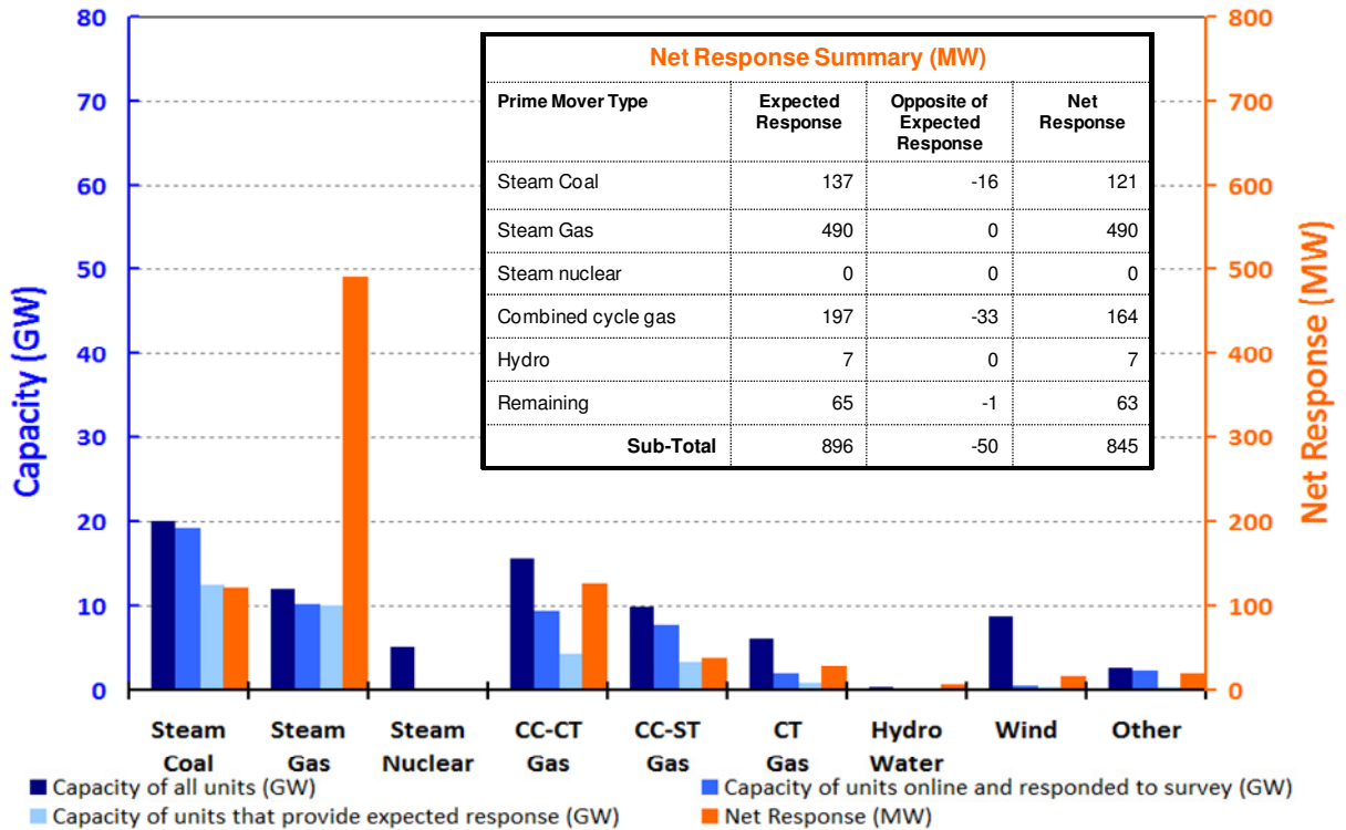
Figure S26 – ERCOT Interconnection Generator Governor Performance
