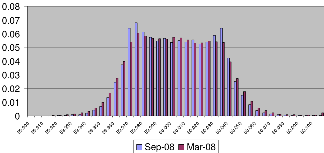
Figure T2 – Frequency Profile for March and September 2008 (in 5 mHz bins)
