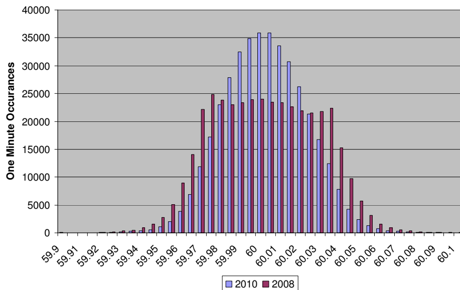
Figure T5 – ERCOT 2010 versus 2008 Frequency Profile (Jan. – Sept.)
