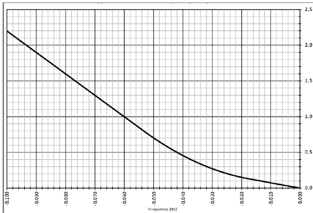
Figure M3: Typical Non-Linear Frequency Response
