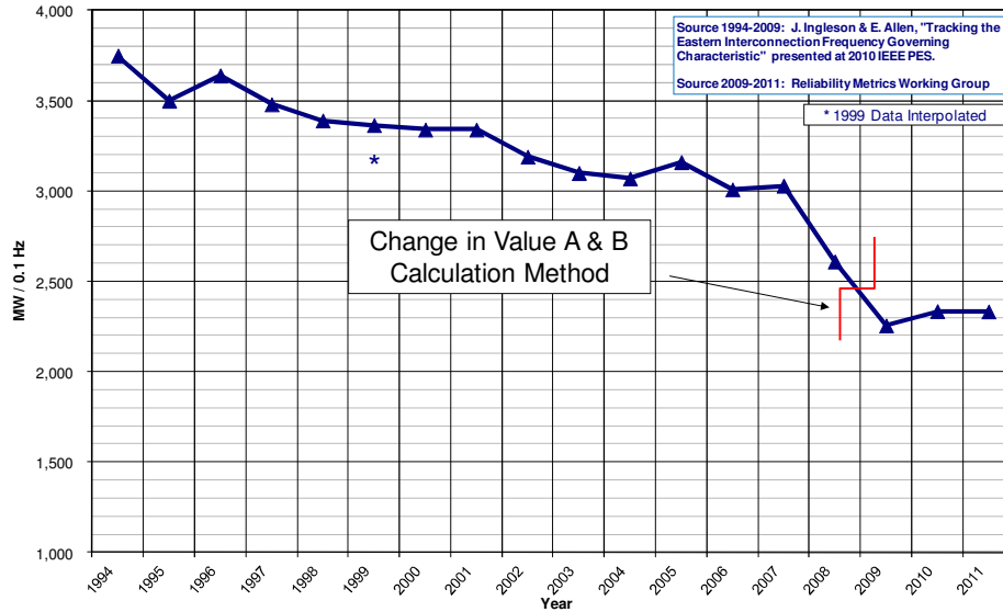
Figure H2 – Updated Eastern Interconnection Mean Primary Frequency Response (May 2012)
