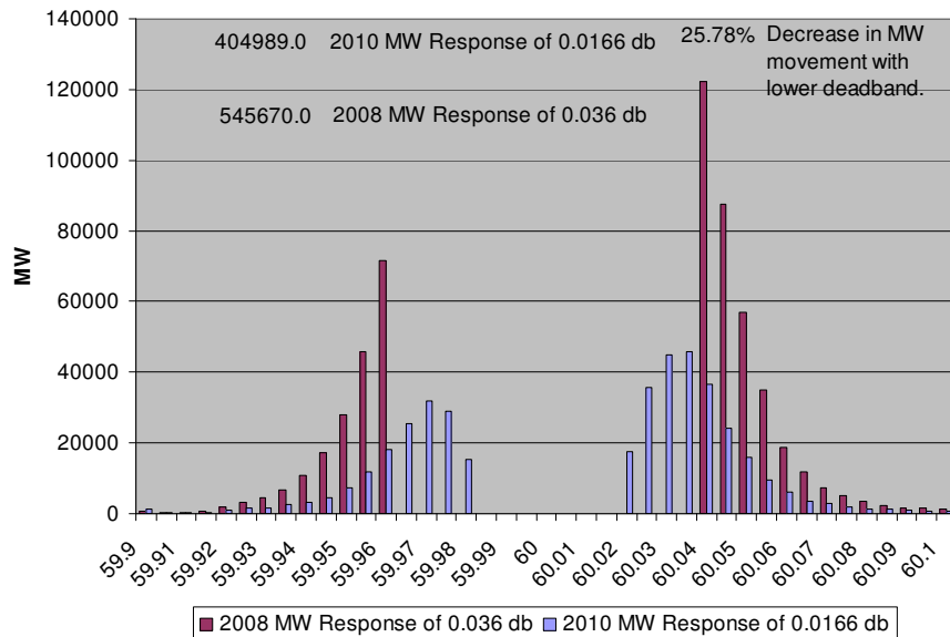
Figure T4 – MW-Minute Movement of a 600 MW Unit with 5% Droop
