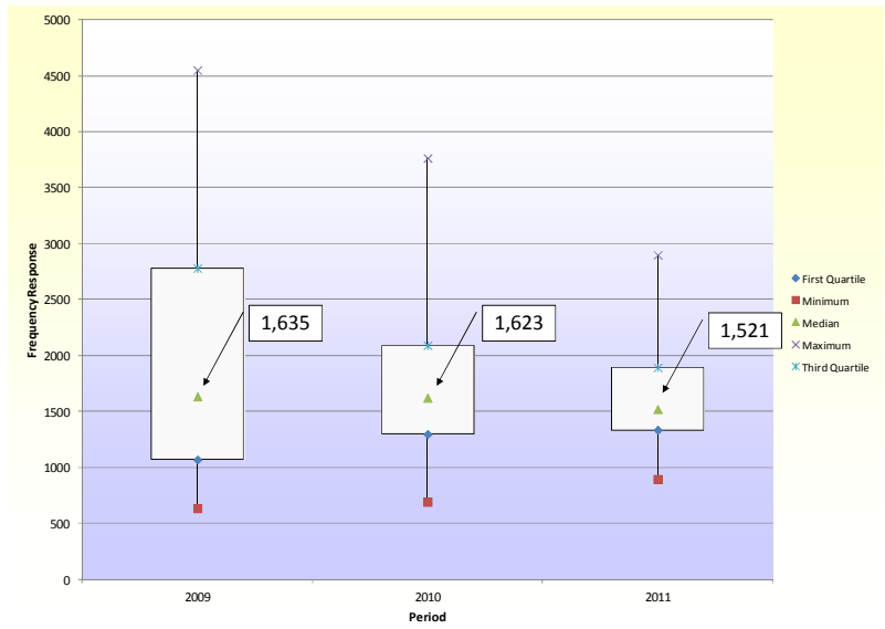
Figure H5 – ERCOT Interconnection Frequency Response Analysis for 2009 to 2011
