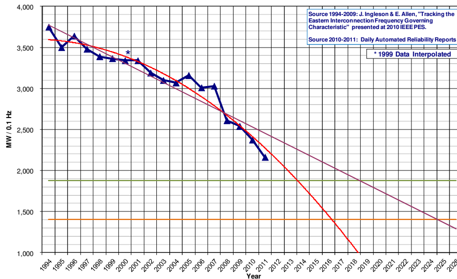
Figure H1 – Eastern Interconnection Mean Primary Frequency Response 12 (March 30, 2012)
