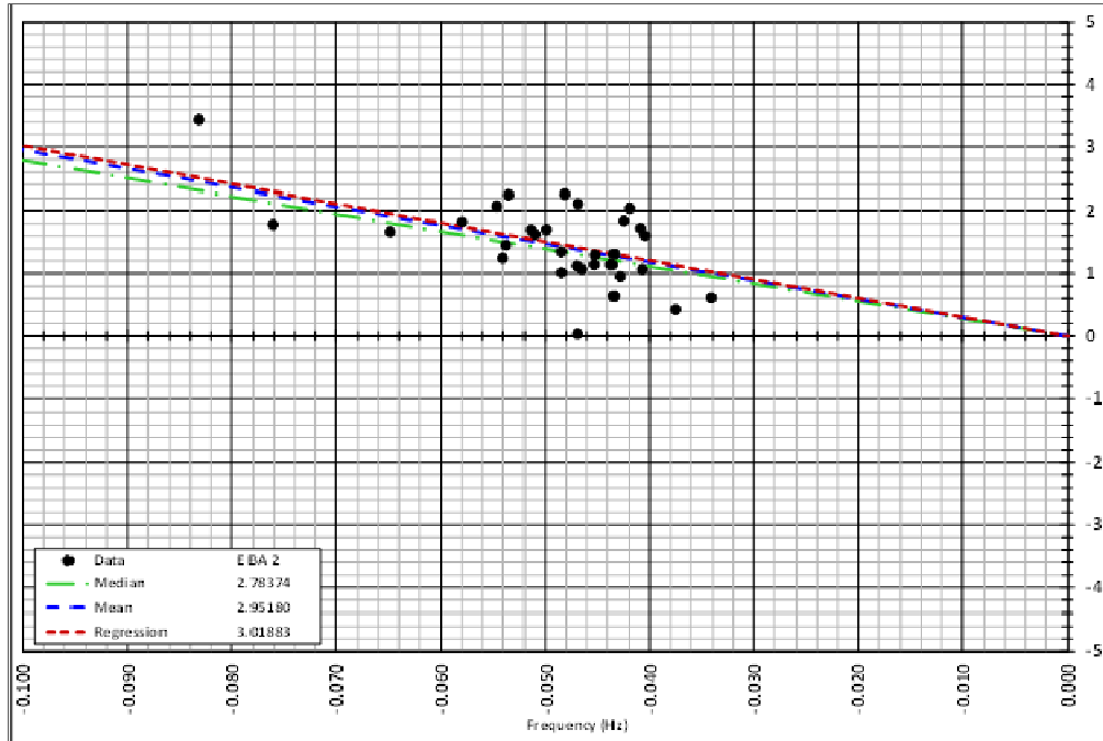
Figure M1: BA with Small Degree of Variability in Measured Frequency Response
