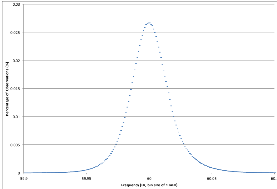
Figure FA3: Québec Interconnection 2010-2011 Frequency Histogram
