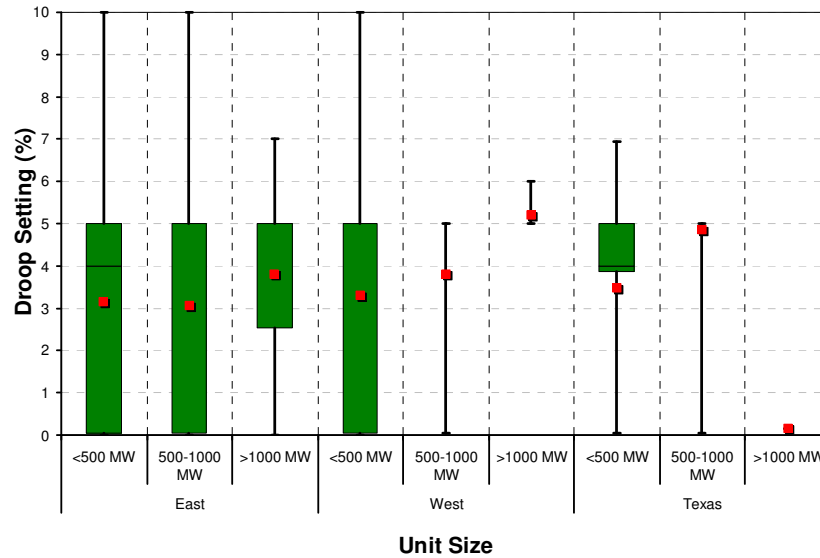
Figure S8 – Range of Governor Droop Settings by Generating Unit Size
