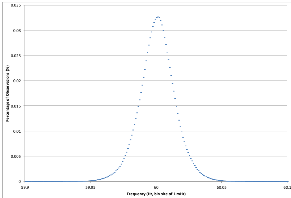
Figure FA2: Western Interconnection 2007-2011 Frequency Histogram
