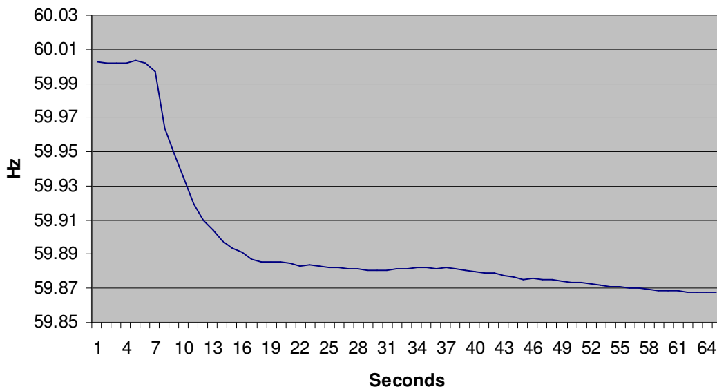
Figure E3 — Interconnection Frequency – August 4, 2007 EI Frequency Excursion
