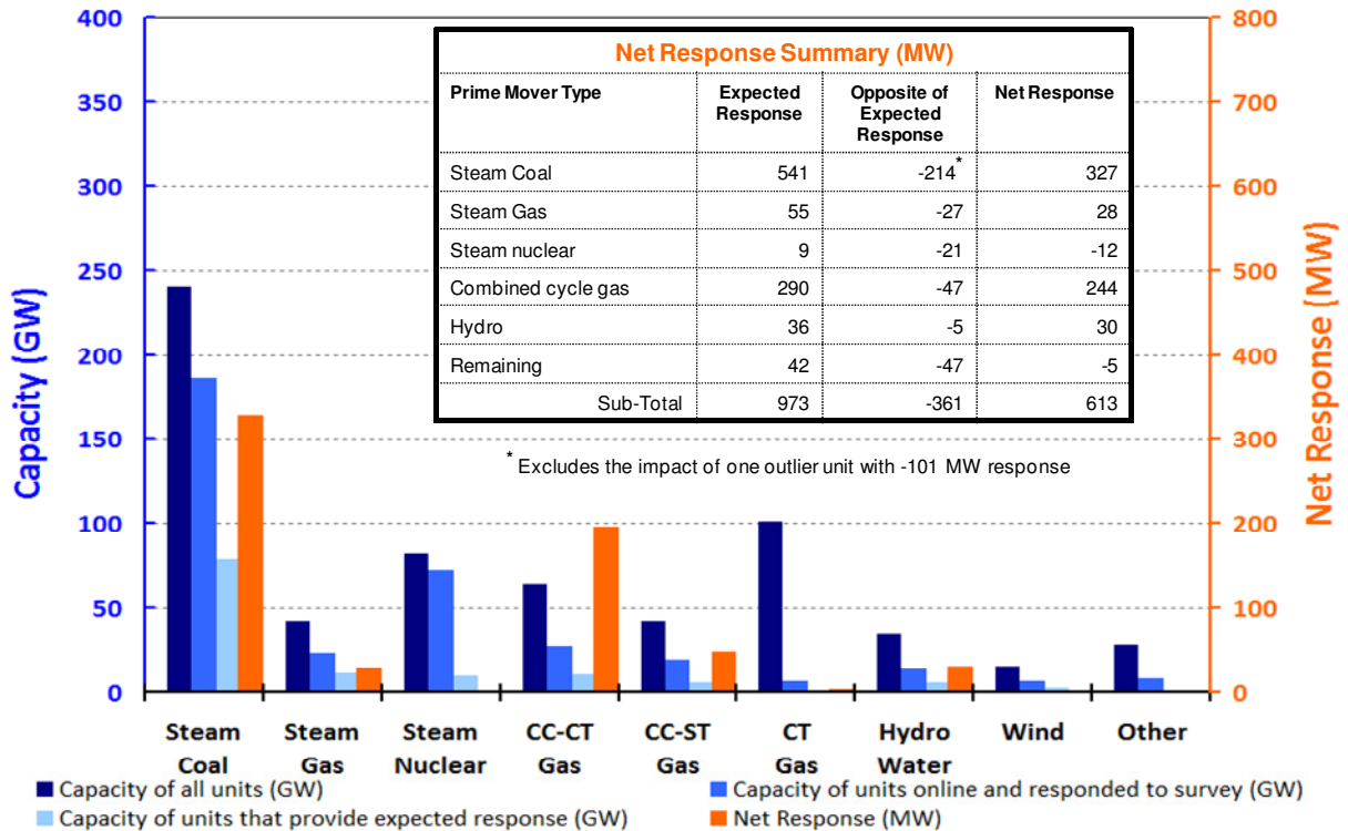
Figure S24 – Eastern Interconnection Generator Governor Performance
