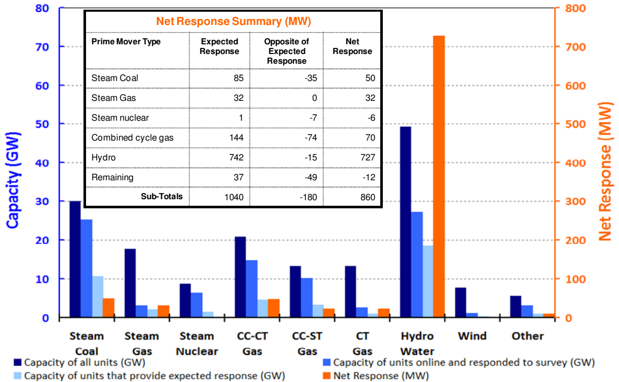
Figure 25 – Western Interconnection Generator Governor Performance
