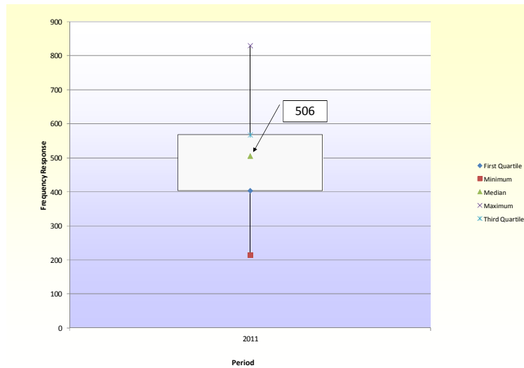
Figure H6 – Quebec Interconnection Frequency Response Analysis for 2011
