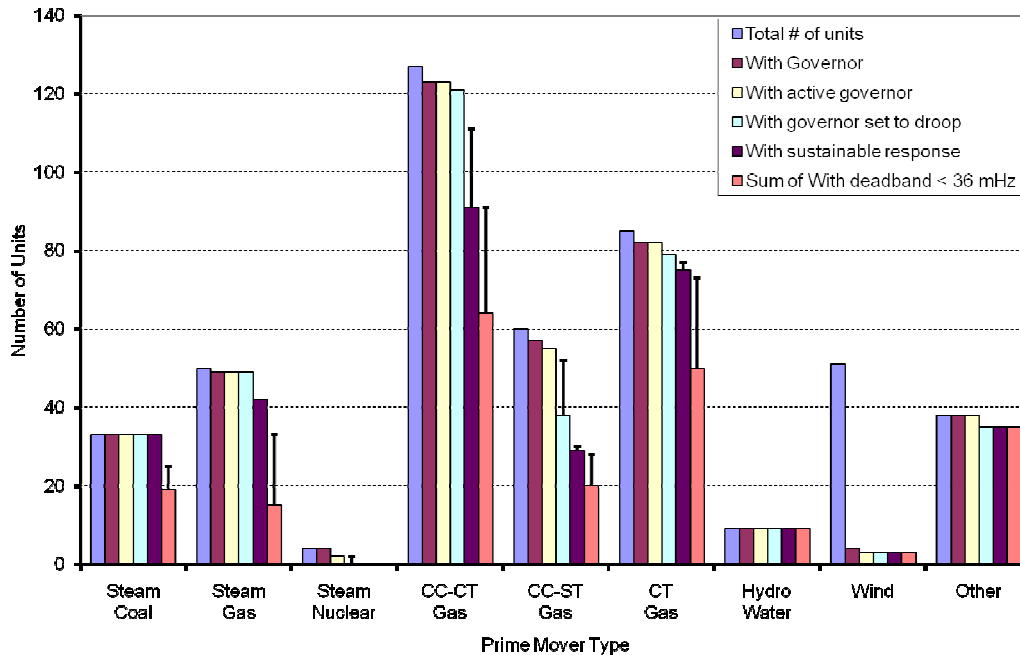
Figure S3 – ERCOT Interconnection Generator Responses
