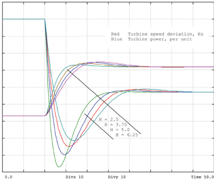
Figure YY: Frequency Response Sensitivity to System Inertia
