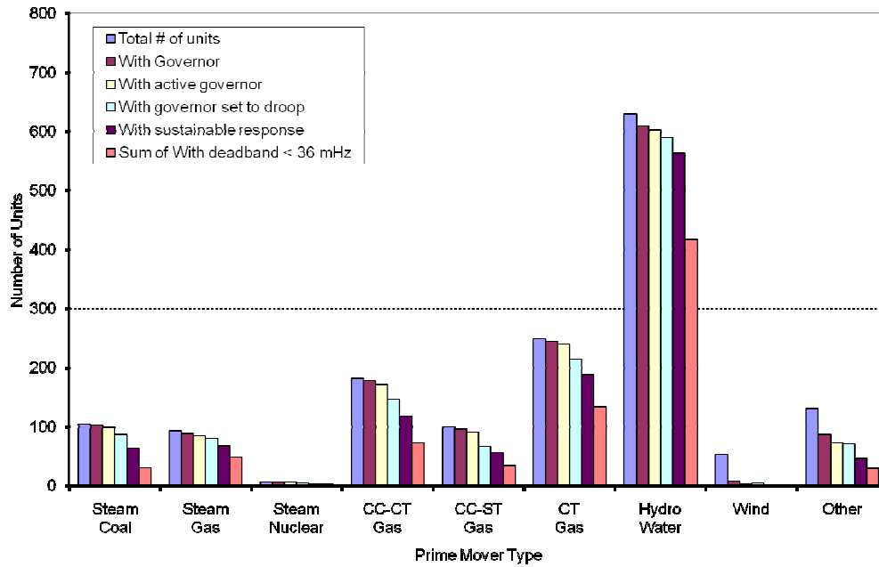
Figure S2 – Western Interconnection Generator Responses
