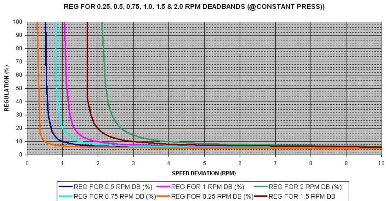
Figure T1 – Regulation versus RPM Deadbands
