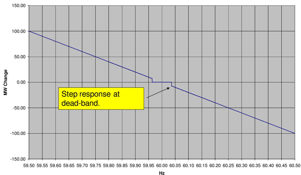
Figure T2A – Frequency Response of 600 MW Unit ±36.0 mHz Deadband and Step Response
