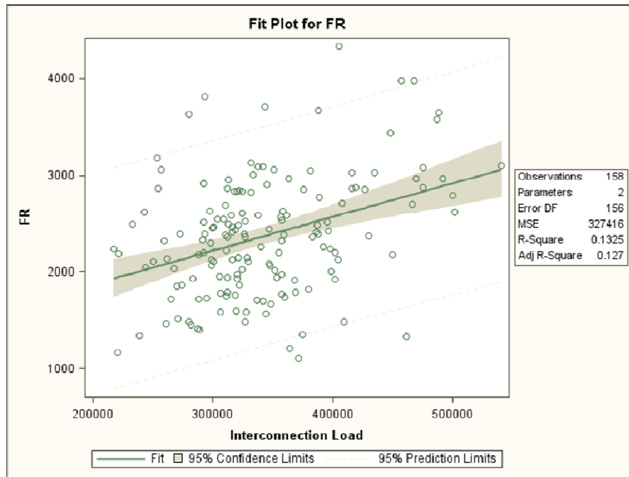
Figure 3: Linear Regression for Frequency Response and Interconnection Load
