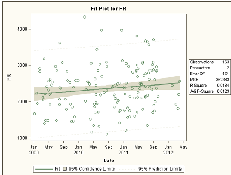
Figure Stat1: Linear Regression Fit Plot for Eastern Interconnection Frequency Response
