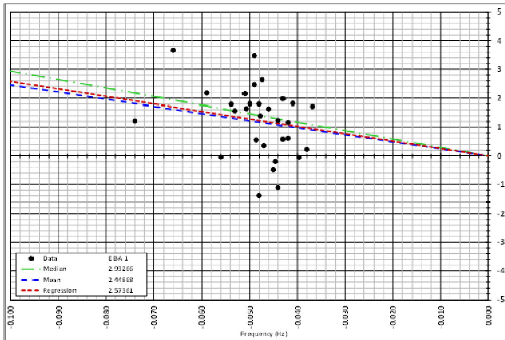
Figure M2: BA with Large Degree of Variability in Measured Frequency Response
