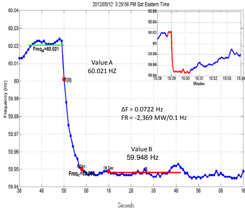
Figure E1 – 3:30 pm Saturday Afternoon 1,711 MW Resource Loss
