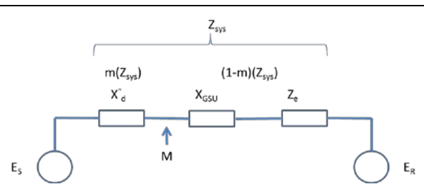
Figure 18: Simple system equivalent impedance diagram to be evaluated. 30
